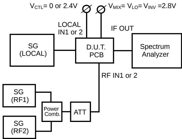
OIP3, IIP3 Measuring Block Diagram
