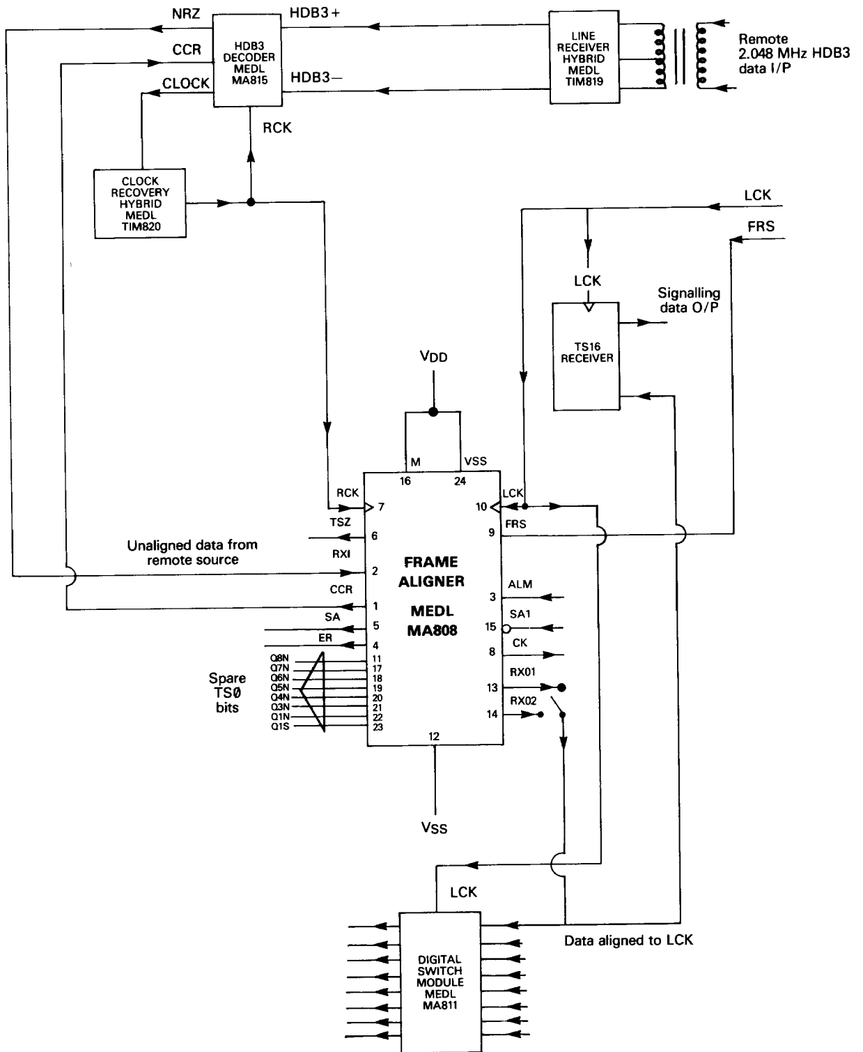
BLOCK DIAGRAM OF A DIGITAL EXCHANGE INCORPORATING THE MA808 IN ENHANCED MODE
