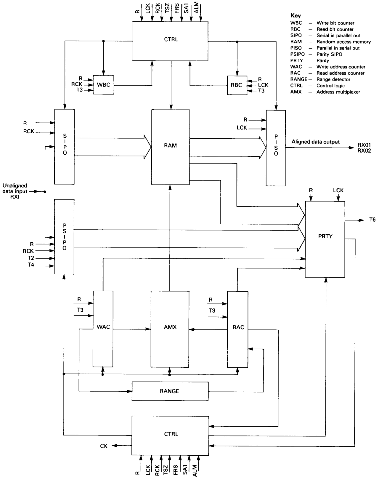
FRAME ALIGNER BLOCK DIAGRAM
