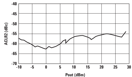
Figure 10. Adjacent Channel Leakage Ratio 2 vs. Output Power.
