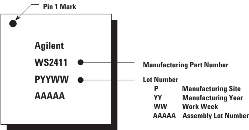
Figure 20. Marking Specification.
