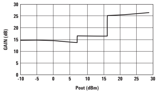
Figure 7. Gain vs. Output Power.
