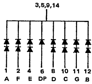
CS-615 COMMON CATHODE NO.7,13 NO PIN
