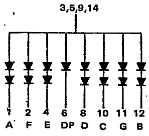
CS-614 COMMON ANODE NO.7,13 NO PIN
