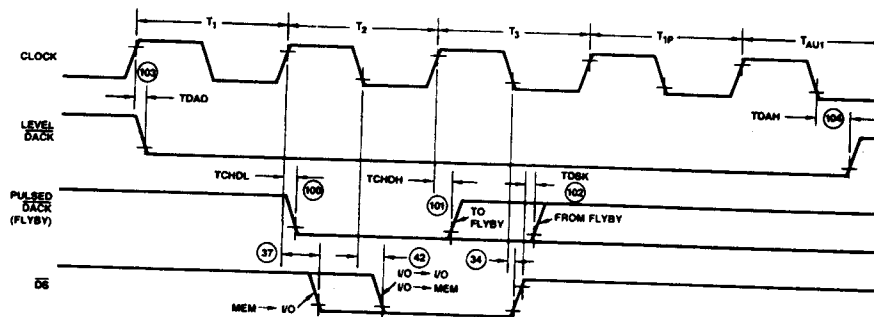
Timing Diagram 18. \overline{\text{DACK}} Timing
