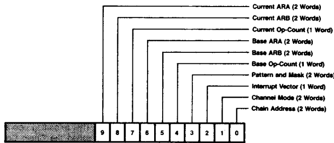
Figure 3. Reload Word
