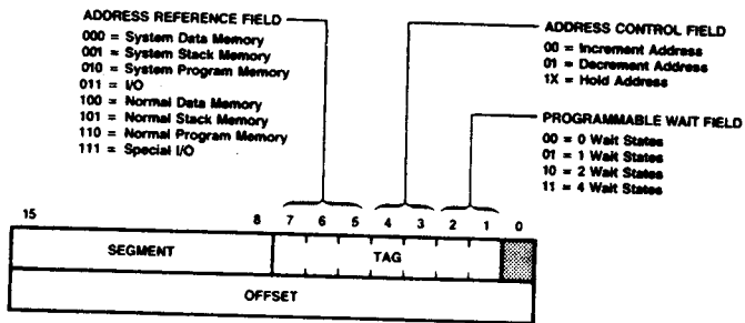
Figure 15. Address Register A and B
