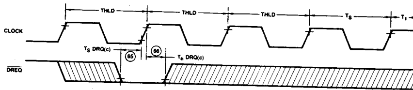
Timing Diagram 17a). Sampling \overline{\text{DREQ}} at the End of Chaining
