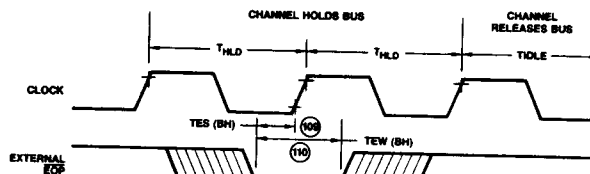
Timing Diagram 19b). Sampling of \overline{\text{EOP}} during Bus Hold
