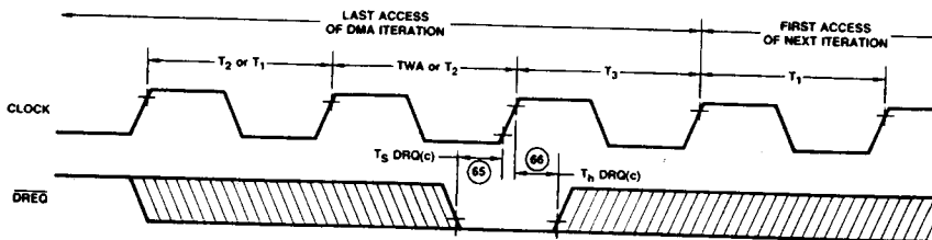
Timing Diagram 17b). Sampling of \overline{\text{DREQ}} While in Bus Hold Mode
