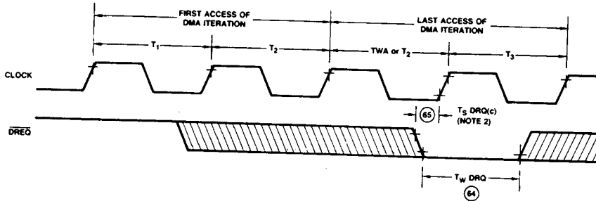
Timing Diagram 16. Sampling \overline{\text{DREQ}} during Single Transfer DMA Operations
