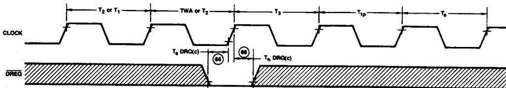
c) Sampling \overline{\text{DREQ}} at the End of Chaining
