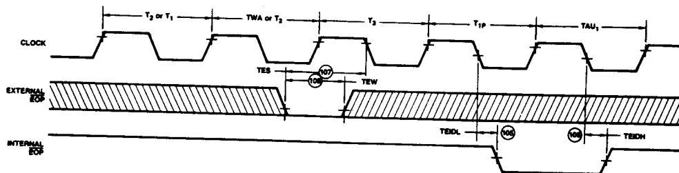
Timing Diagram 19a). \overline{\text{EOP}} Sampling and Generation during DMA Operations
