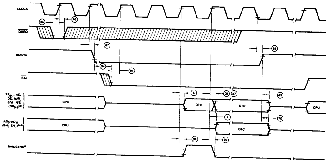
Timing Diagram 13. Bus Exchange Timing
