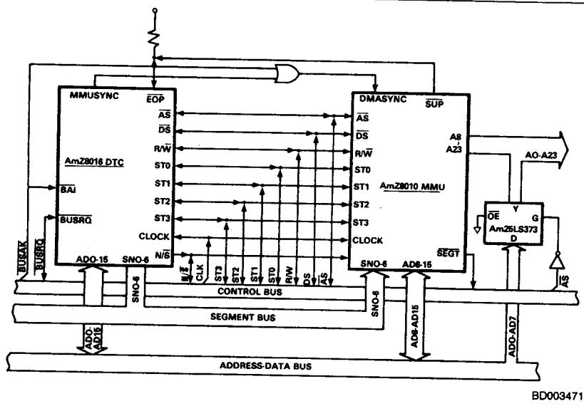
Figure 24. AmZ8016 DTC to AmZ8010 MMU Interface Configuration
