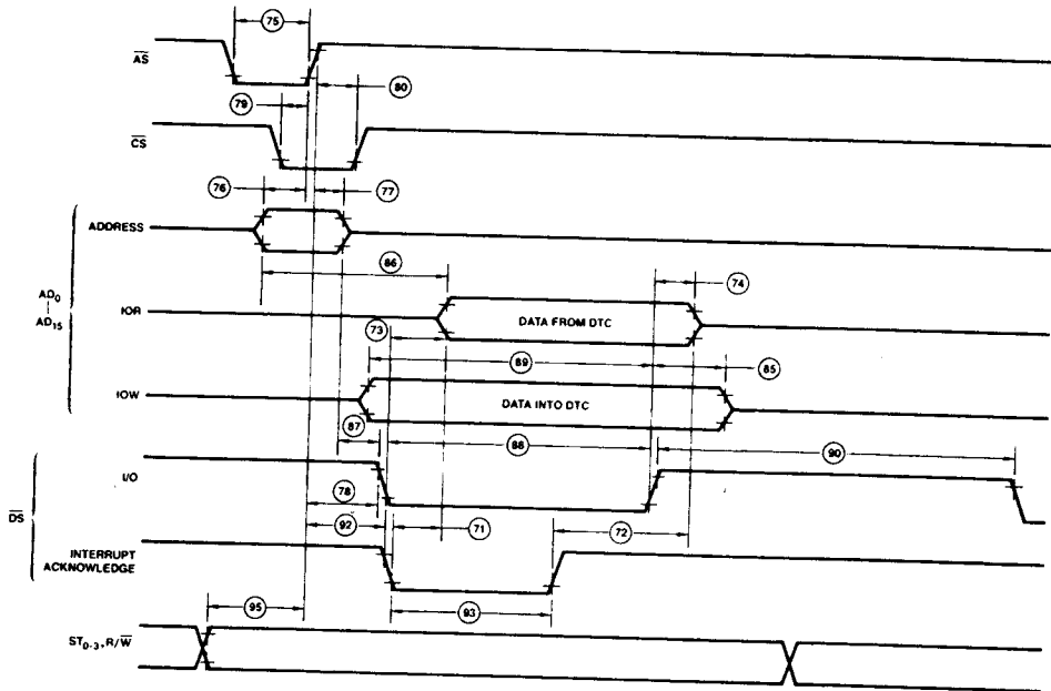
Timing Diagram 12. AC Timing when DTC is Bus Slave
