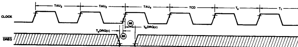
d) Sampling \overline{\text{DREQ}} at the End of Base-to-Current Reloading
