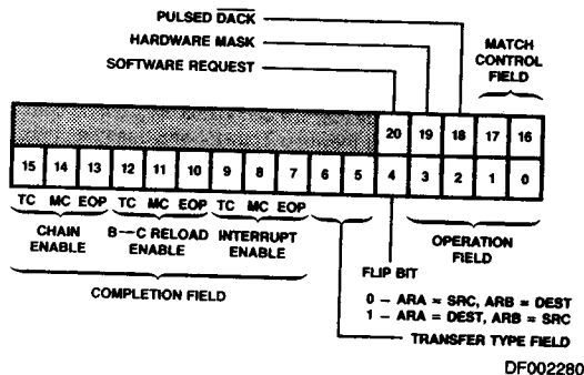
Figure 18. Channel Mode Register
