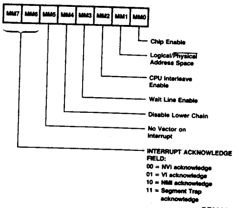
Figure 13. Master Mode Register
