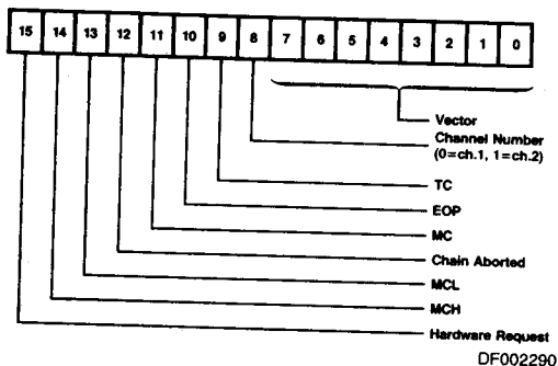
Figure 17. Interrupt Save Register
