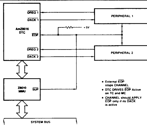
Figure 8. EOP Connection
