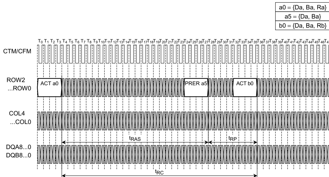
Figure 14. Precharge with PRER Command in ROWR Packet
