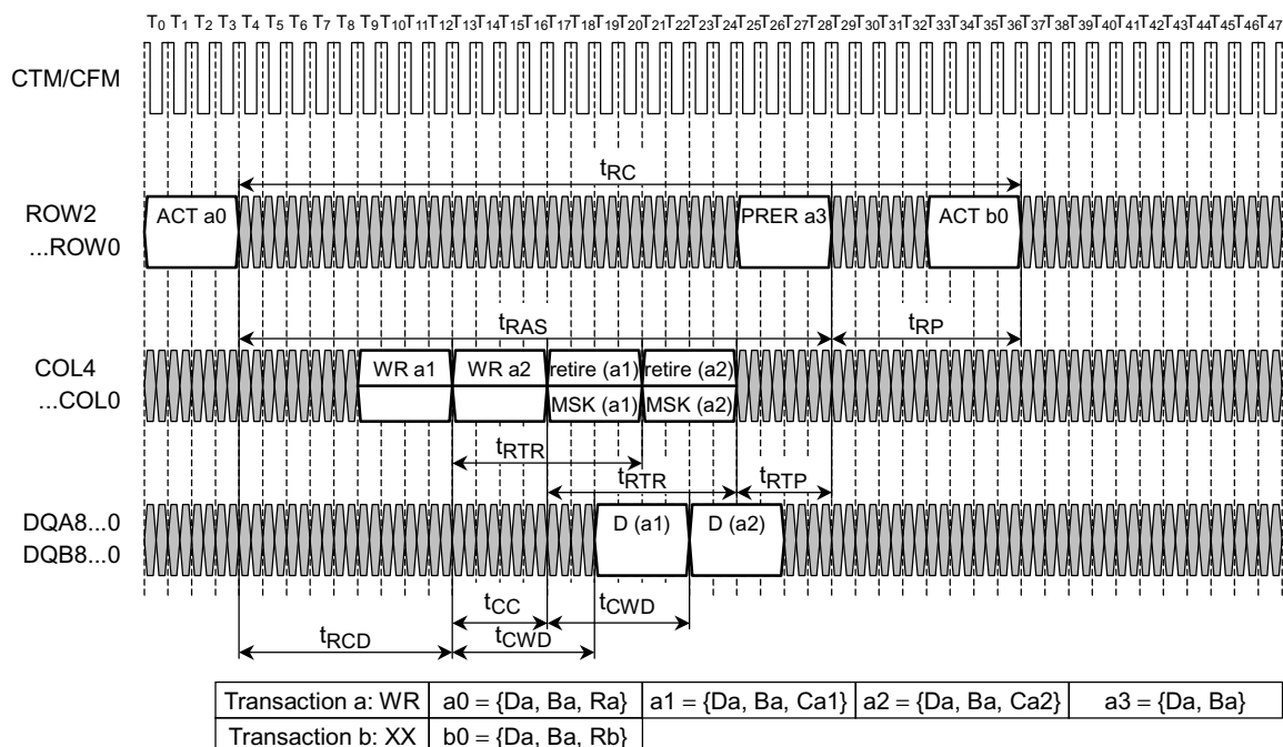
Figure 17. Write Transaction Example
