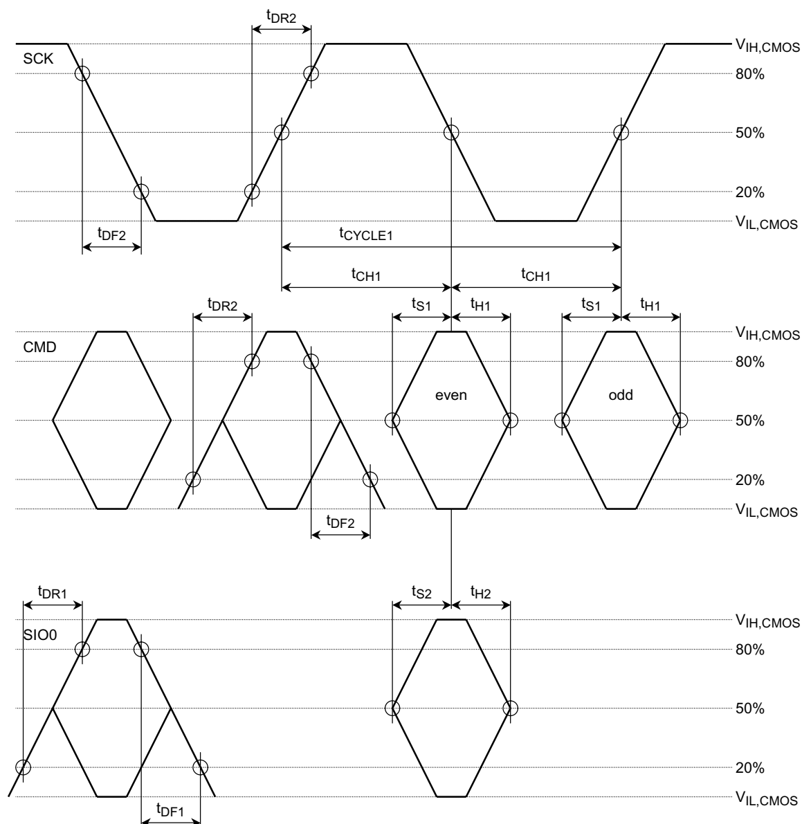
Figure 44. CMOS Timing-Data Signals for Receive
