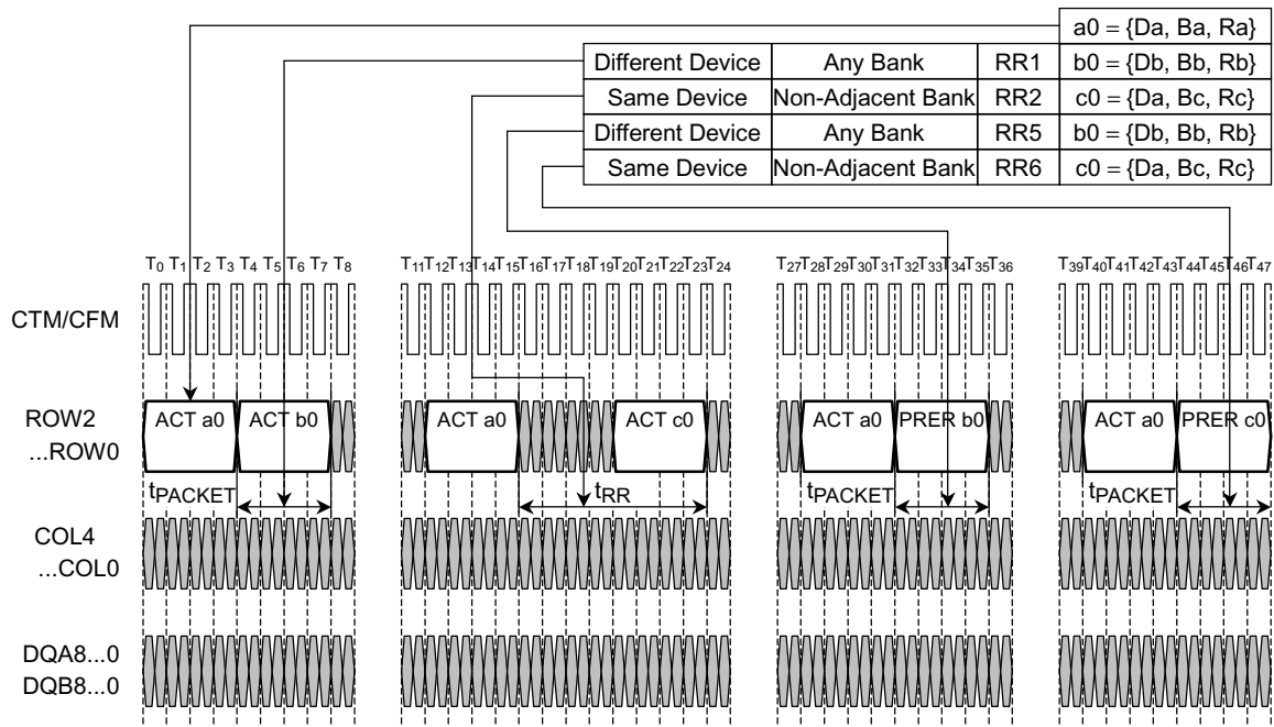
Figure 12. ROW Packet Examples
