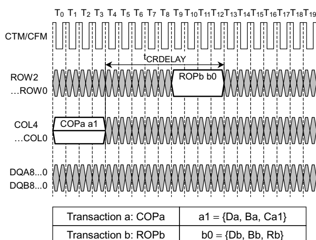
Figure 10. COL-to-ROW Packet Interaction Timing
