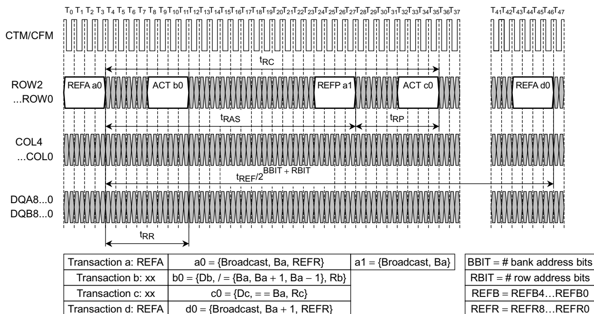
Figure 38 - (1). REFA/REFP Refresh Transaction Example
