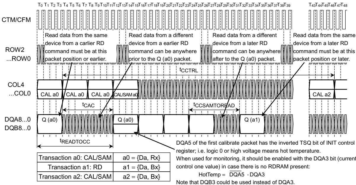
Figure 39. Current Control CAL/SAM transaction Example
