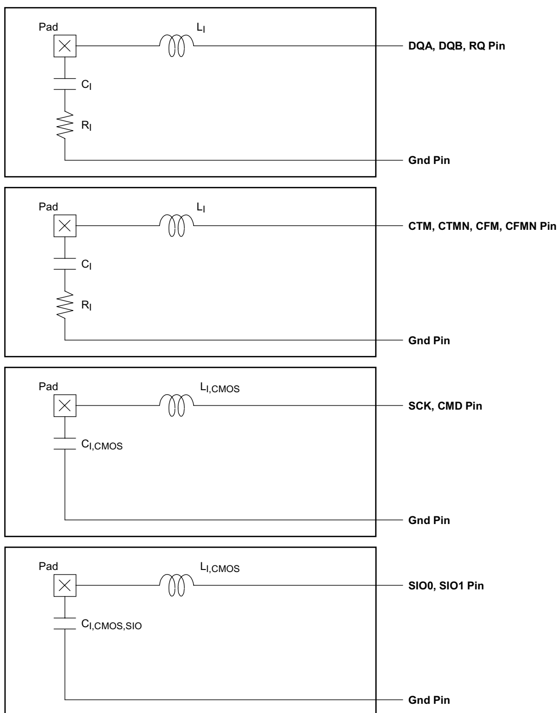
Figure 48. Equivalent Load Circuit for RSL Pins
