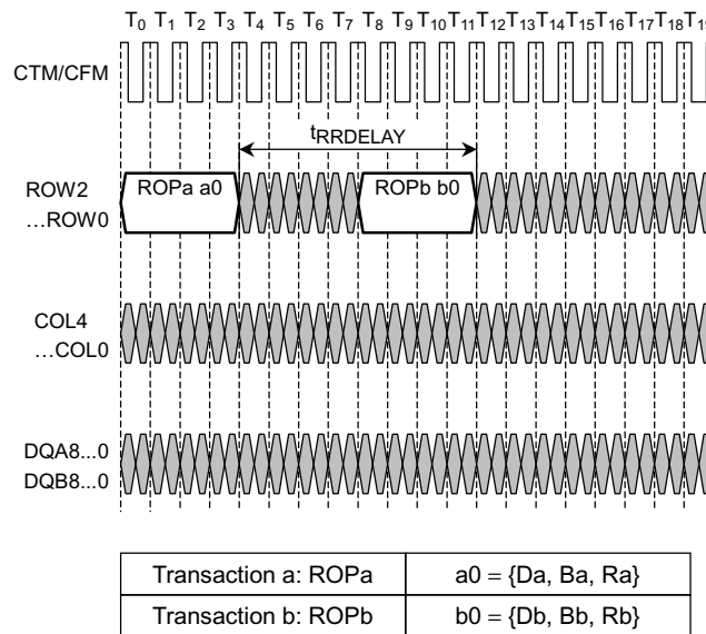
Figure 7. ROW-to-ROW Packet interaction-Timing
