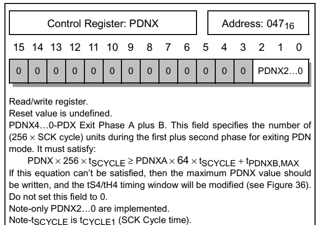
Figure 30. Control Registers
