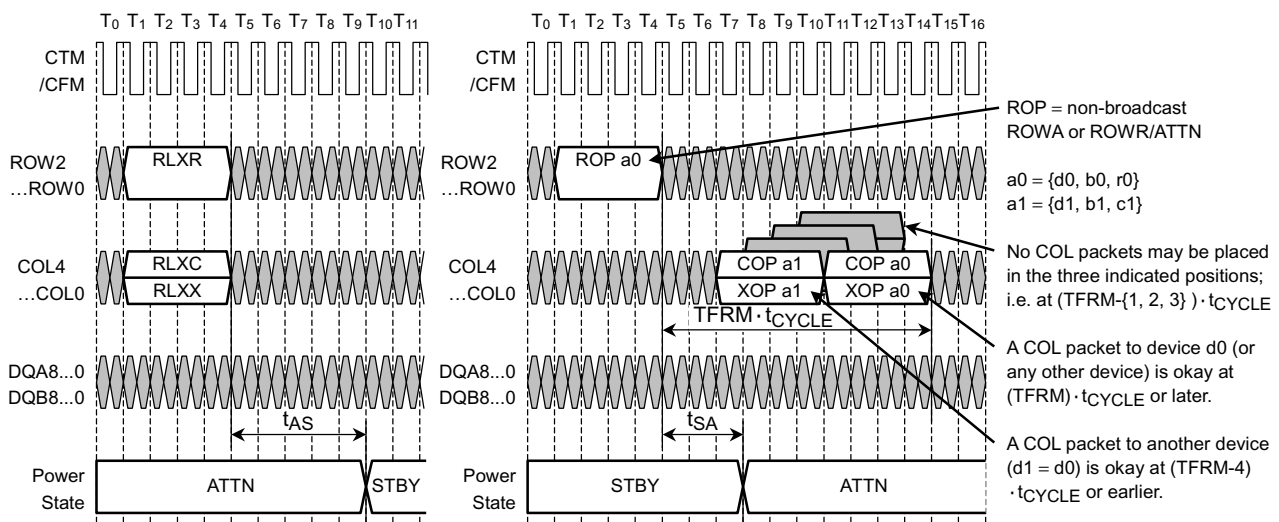
Figure 34. STBY Entry (left) and STBY Exit (right)
