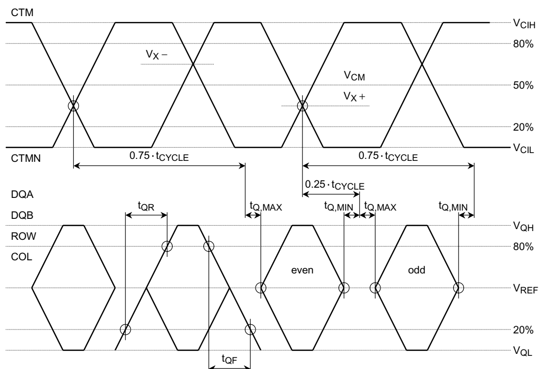
Figure 43. RSL Timing-Data Signals for Transmit
