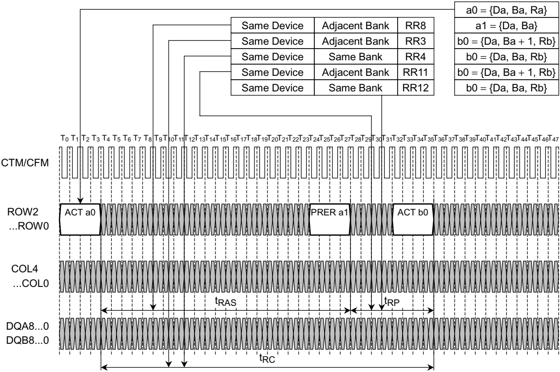
Figure 11. ROW Packet Example
