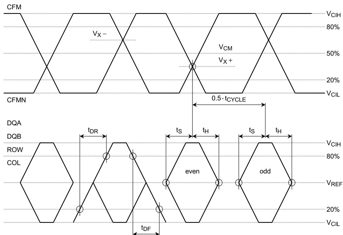
Figure 42. RSL Timing-Data Signals for Receive
