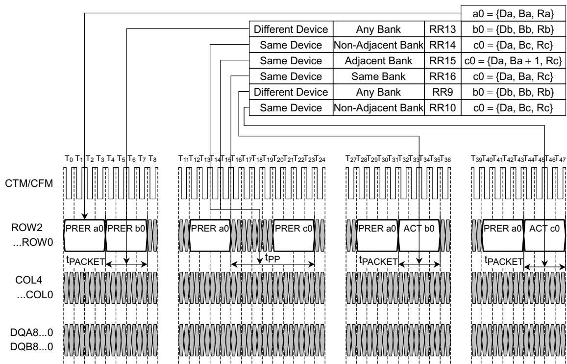
Figure 13. ROW Packet Examples
