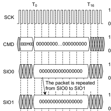
Figure 27. SIO Reset Sequence
