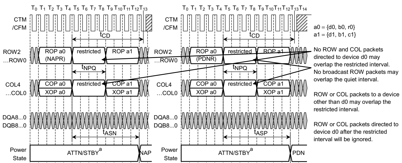
Figure 35. NAP Entry (left) and PDN Entry (right)
