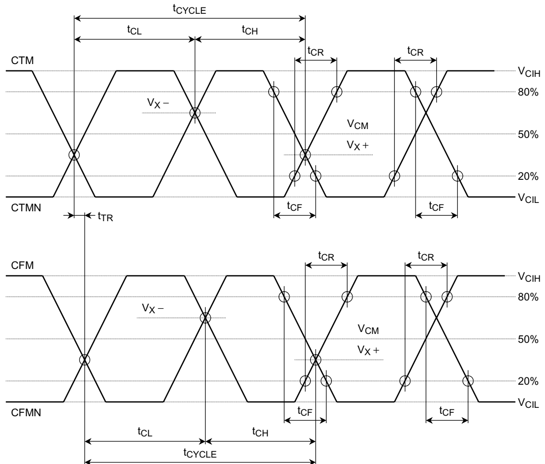
Figure 41. RSL Timing-Clock Signals
