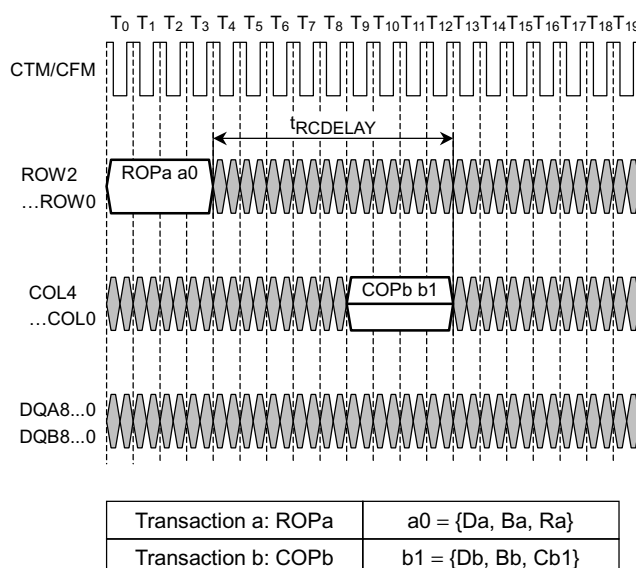
Figure 8. ROW-to-COL Packet Interaction Timing
