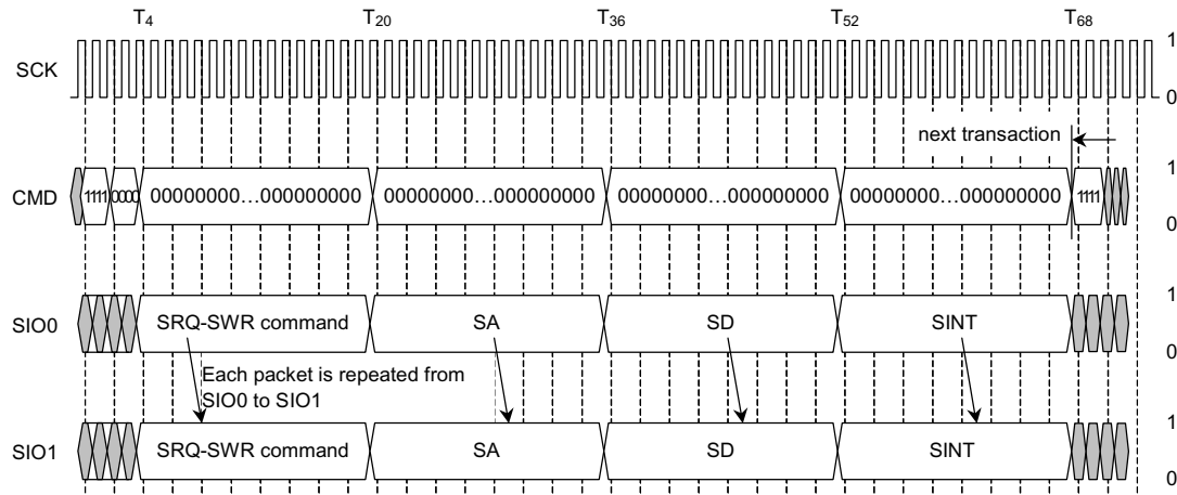
Figure 24. Serial Write (SWR) Transaction to Control Register
