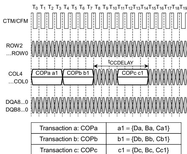
Figure 9. COL-to-COL Packet Interaction Timing
