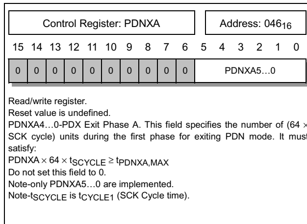
Figure 30. Control Registers
