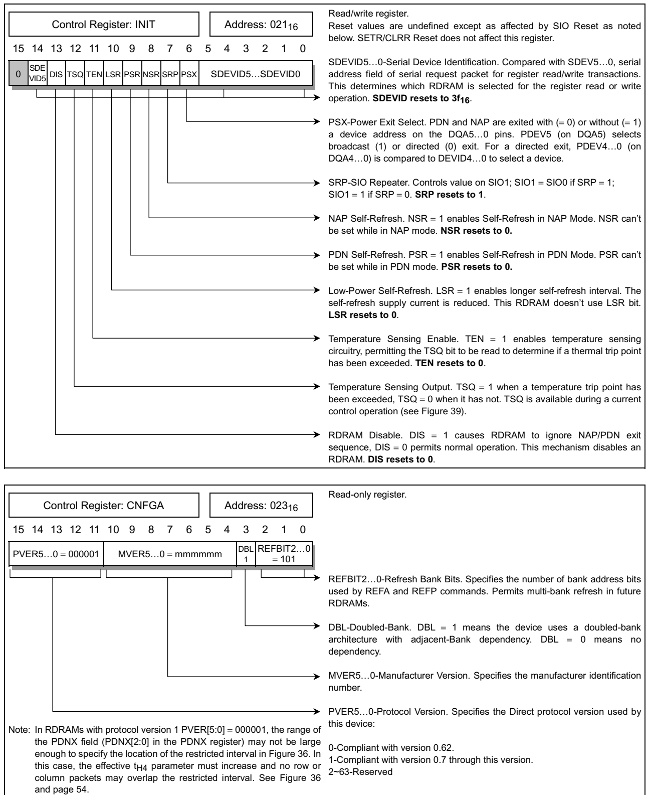
Figure 28. Control Registers
