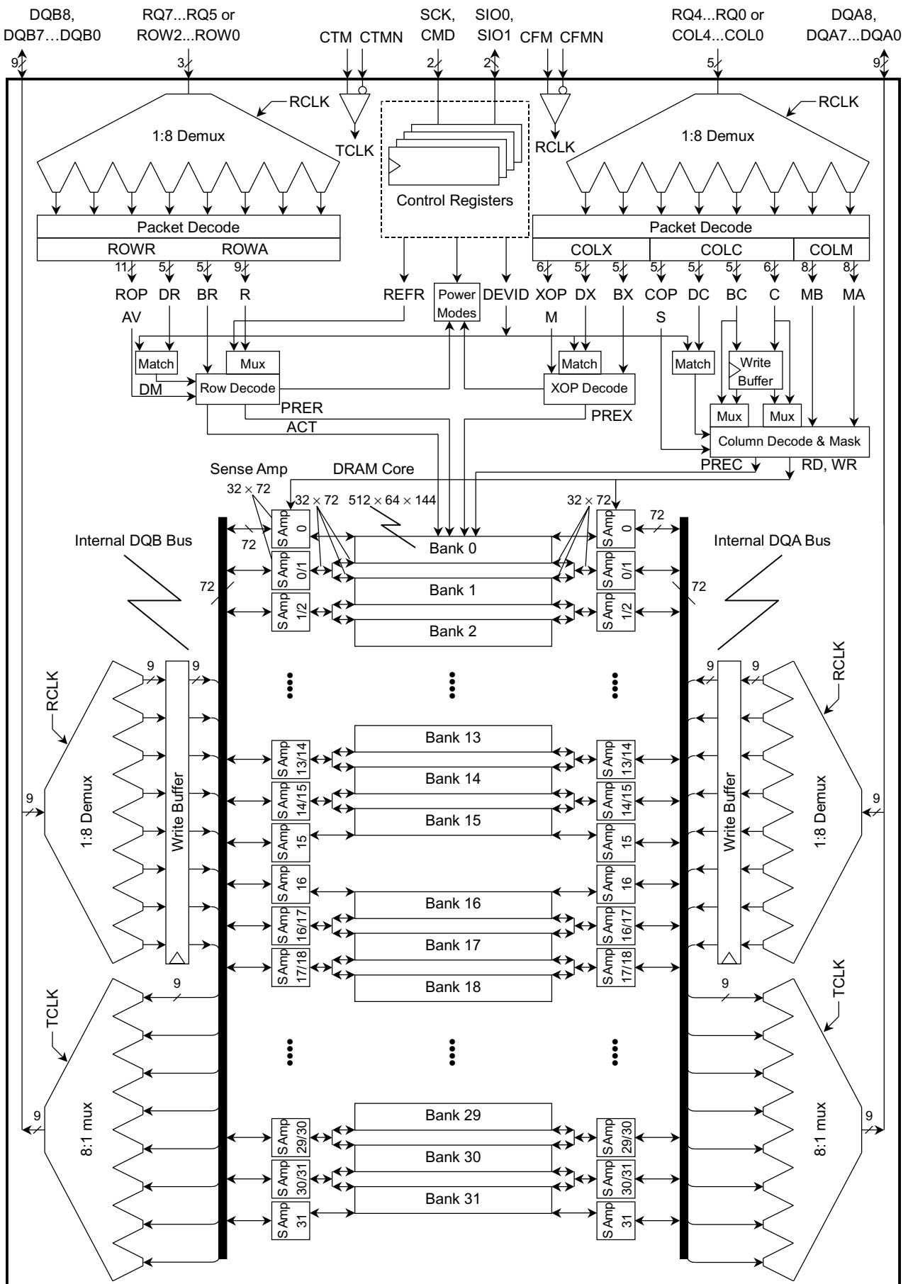
Figure 3. 128/144-Mbit Direct RDRAM Block Diagram
