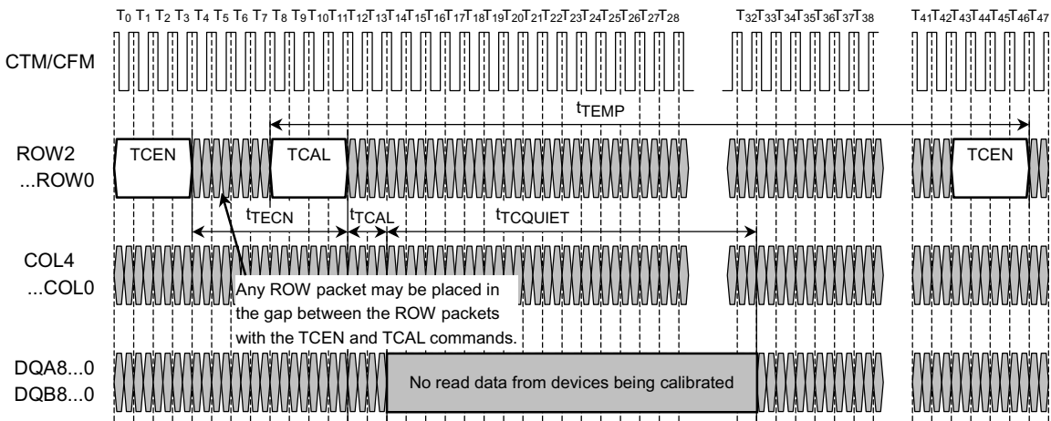
Figure 40. Temperature Calibration (TCEN-TCAL) Transitions to RDRAM
