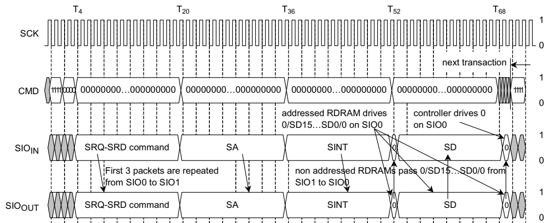
Figure 25. Serial Read (SRD) Transaction to Control Register
