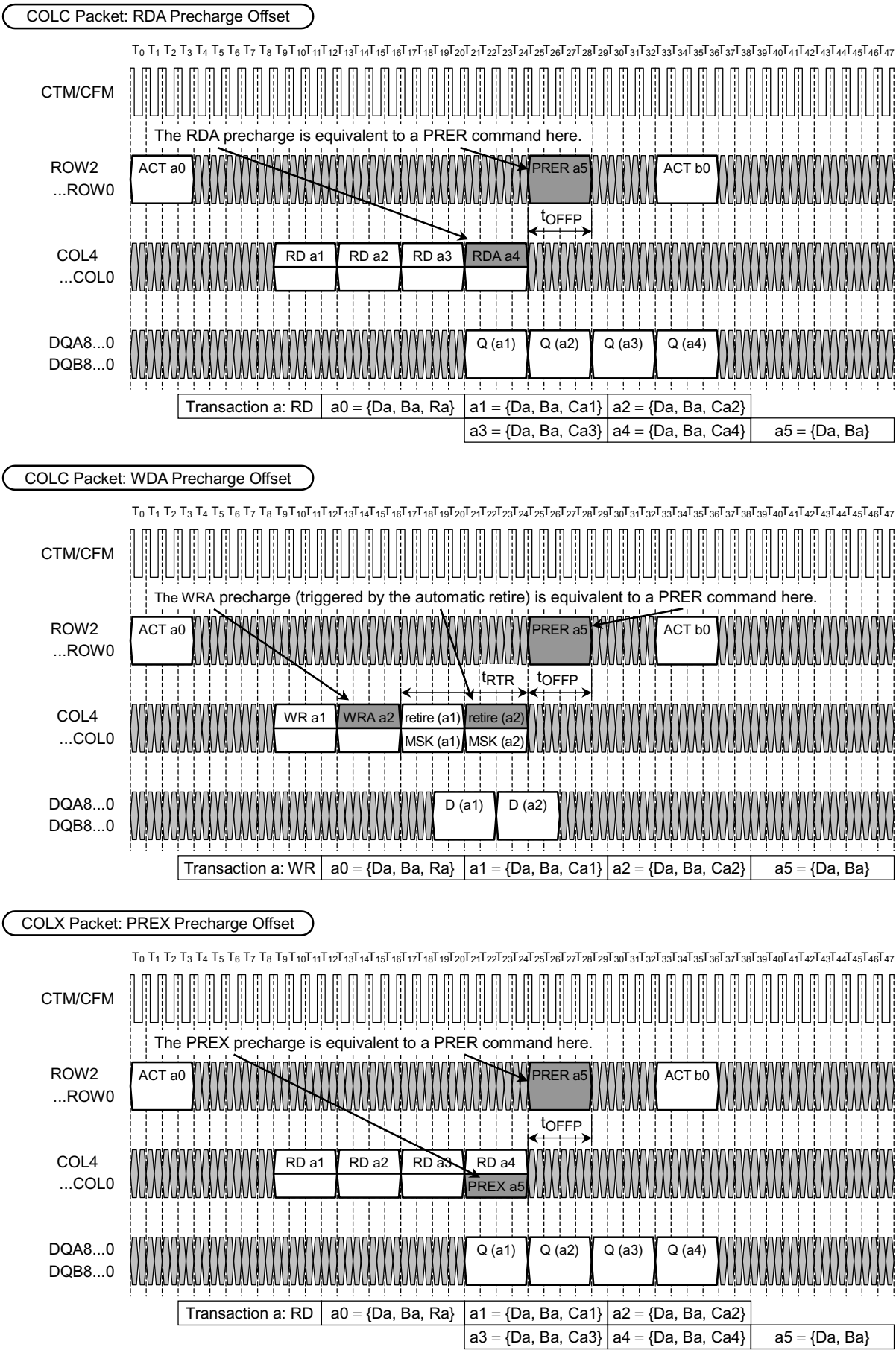
Figure 15. Offsets for Alternative Precharge Mechanisms
