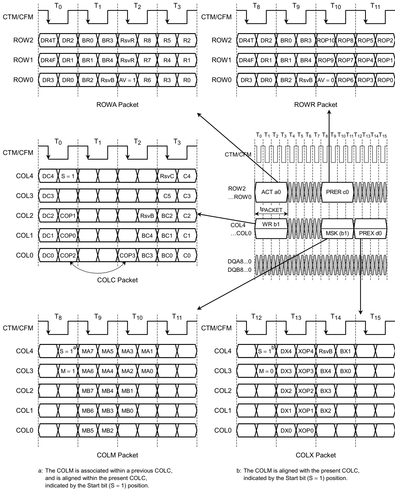
Figure 4. Packet Formats
