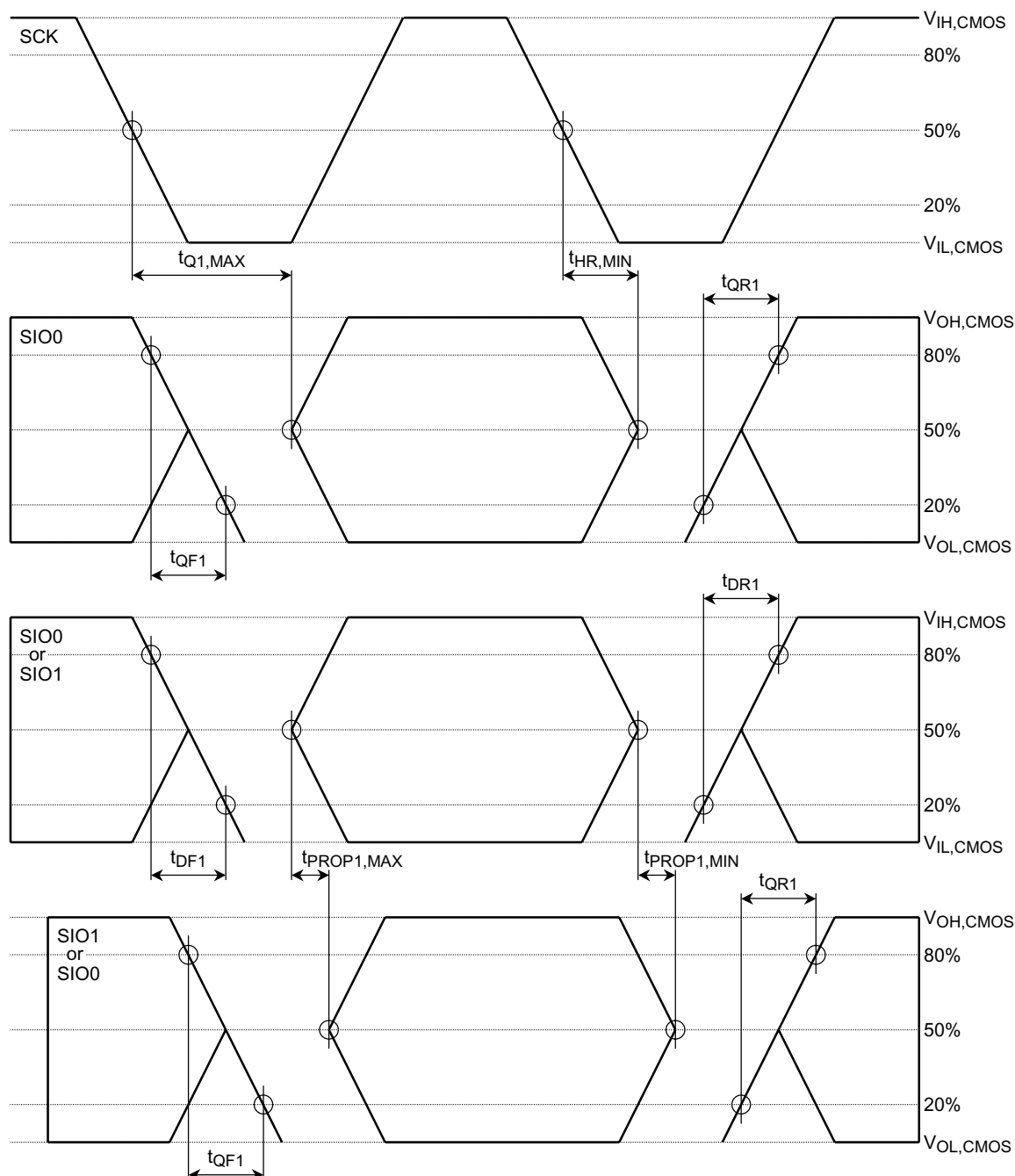
Figure 46. CMOS Timing-Data Signals for Transmit
