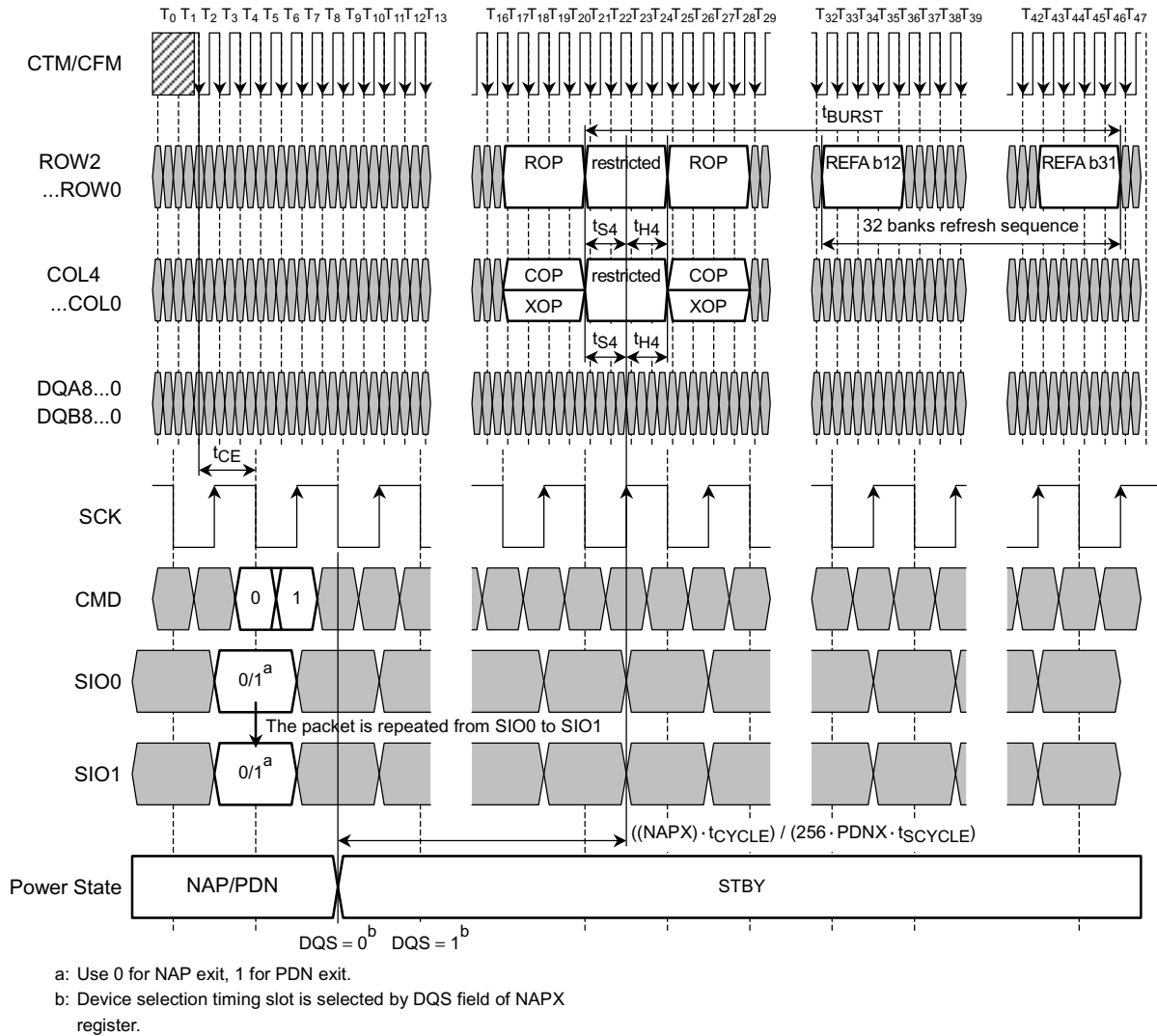
Figure 38 - (2). NAP/PDN Exit-tBURST Requirement
