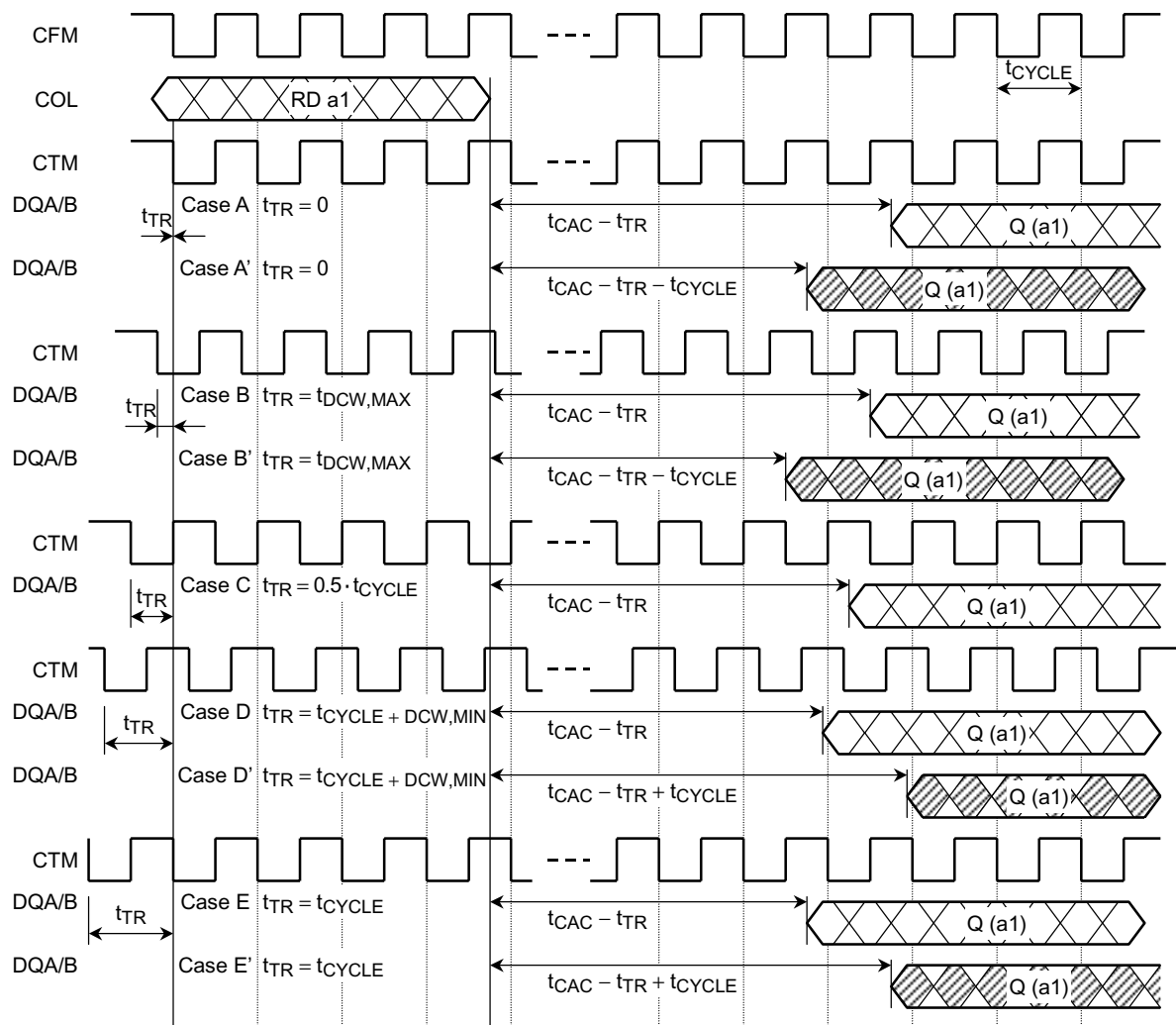
Figure 47. RSL Transmit-Crossing Read Domains
