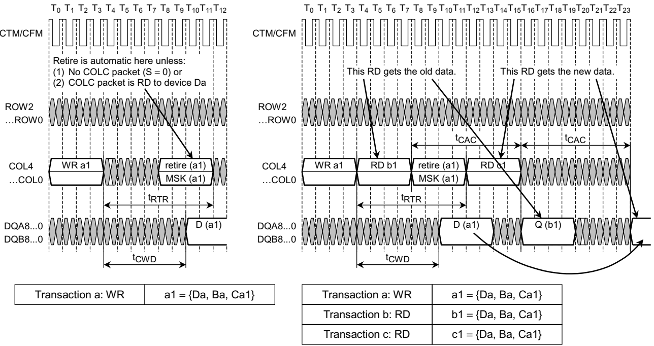
Figure 18. Normal Retire (left) and Retire/Read Ordering (right)
