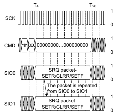
Figure 26. SETR, CLRR, SETF Transaction
