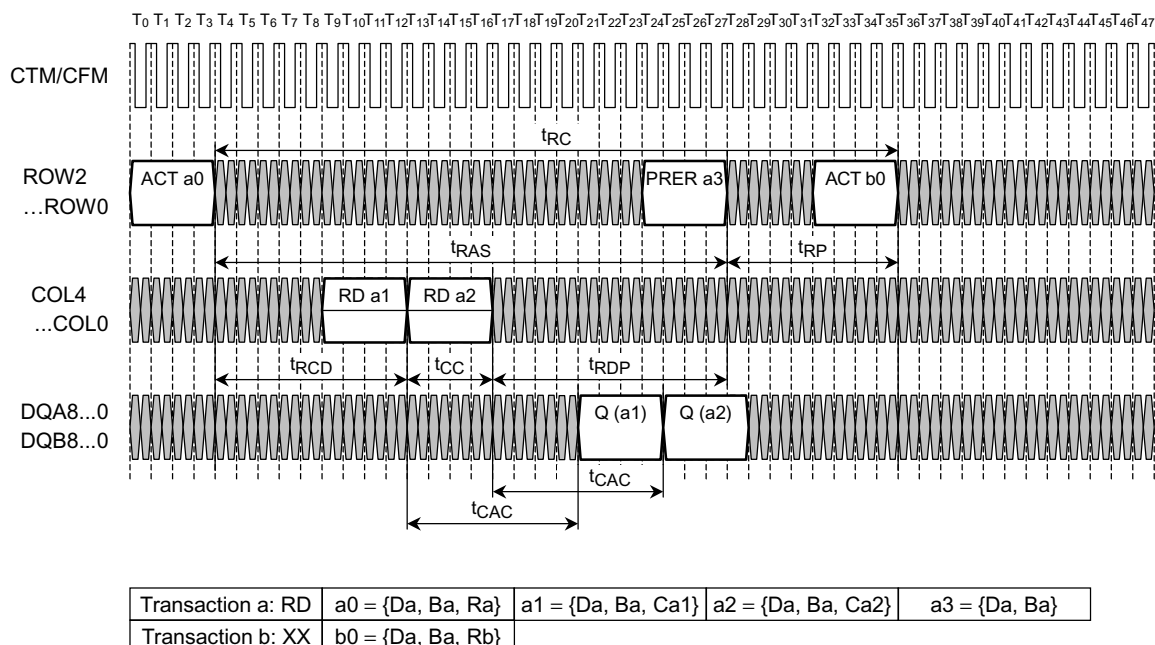
Figure 16. Read Transaction Example
