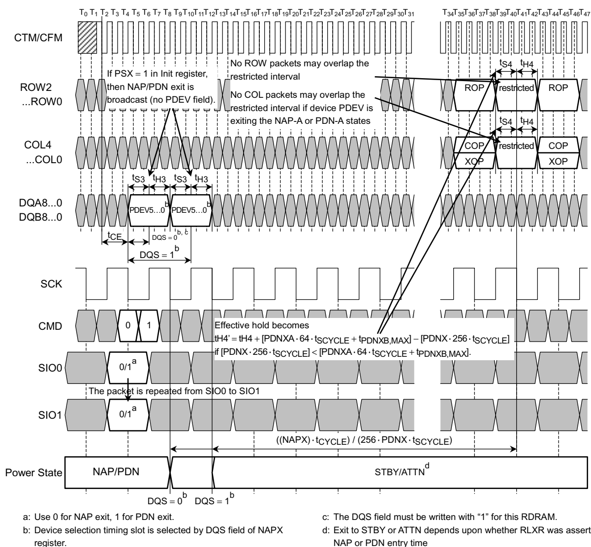
Figure 36. NAP and PDN Exit
