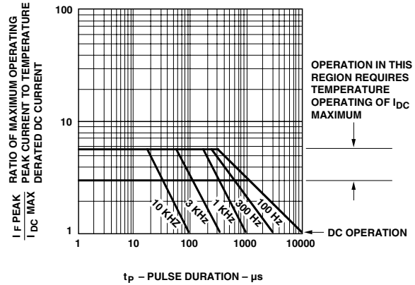
Figure 6. Maximum Tolerable Peak Current vs. Pulse Duration – Yellow.
