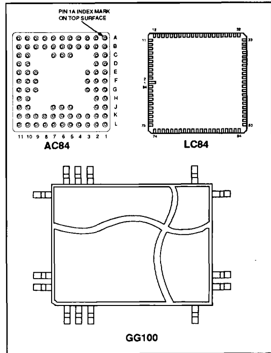
Fig.1 Pin connections - bottom view
