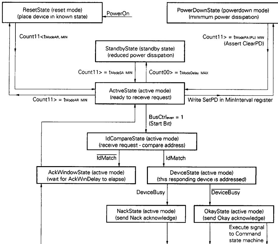
Figure 6-1. Frame State Machine - State Diagram
