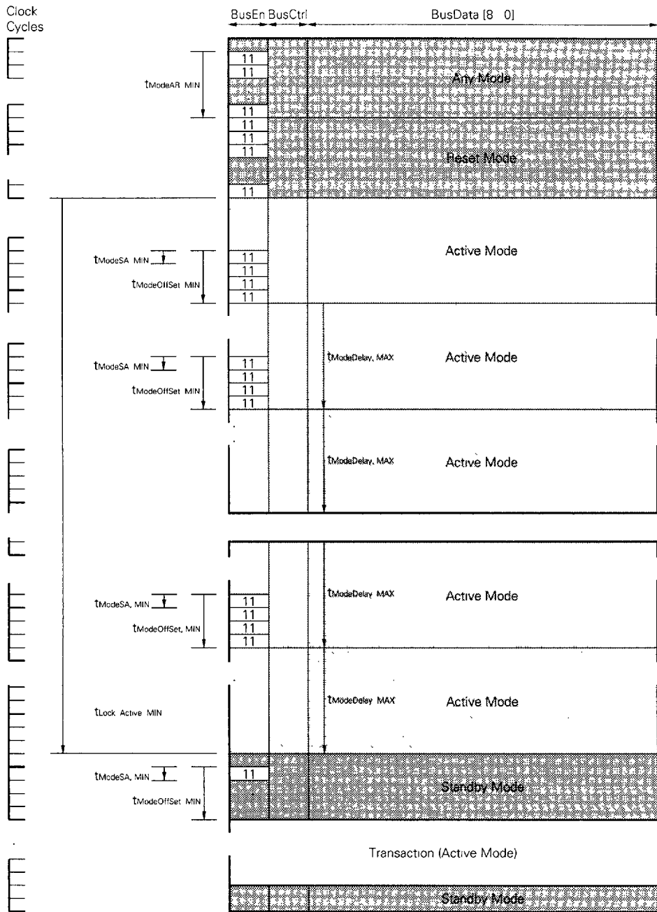
Figure 6-5. ResetMode to ActiveMode Transition
