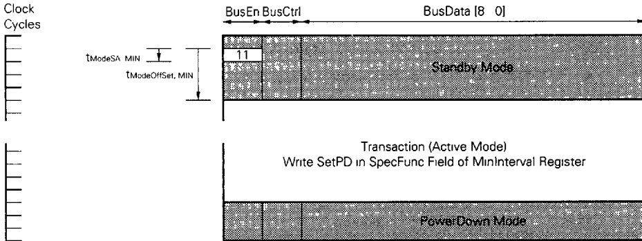
Figure 6-2. ActiveMode to PowerDownMode Transition
