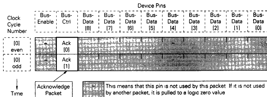
Figure 5-2. Acknowledge Packet Format
