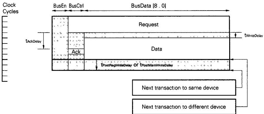
Figure 7-2. Write Transaction
