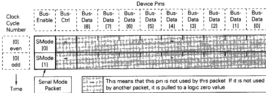
Figure 5-7. Serial Mode Packet Format
