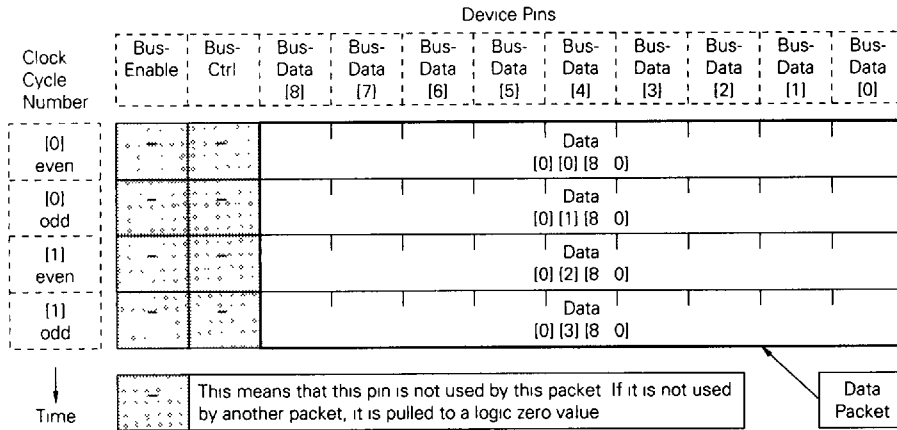
Figure 5-3. Data Packet Format (Register Space)
