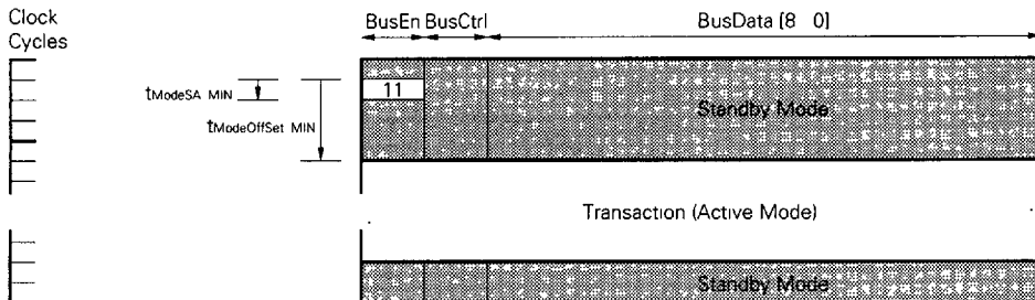
Figure 6-4. ActiveMode/StandbyMode Transition - Early Transaction
