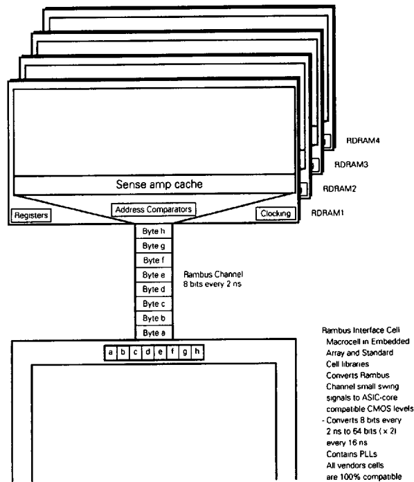
Figure 3-1. Converting the Channel Data Rate
