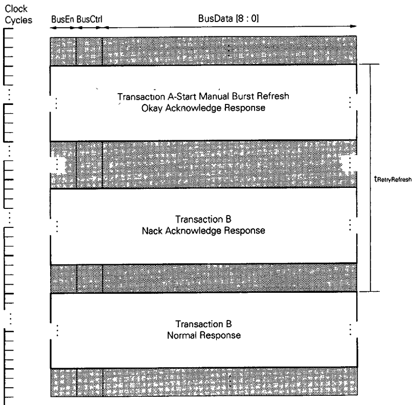
Figure 8-2. Transaction Holdoff Due to Burst Refresh
