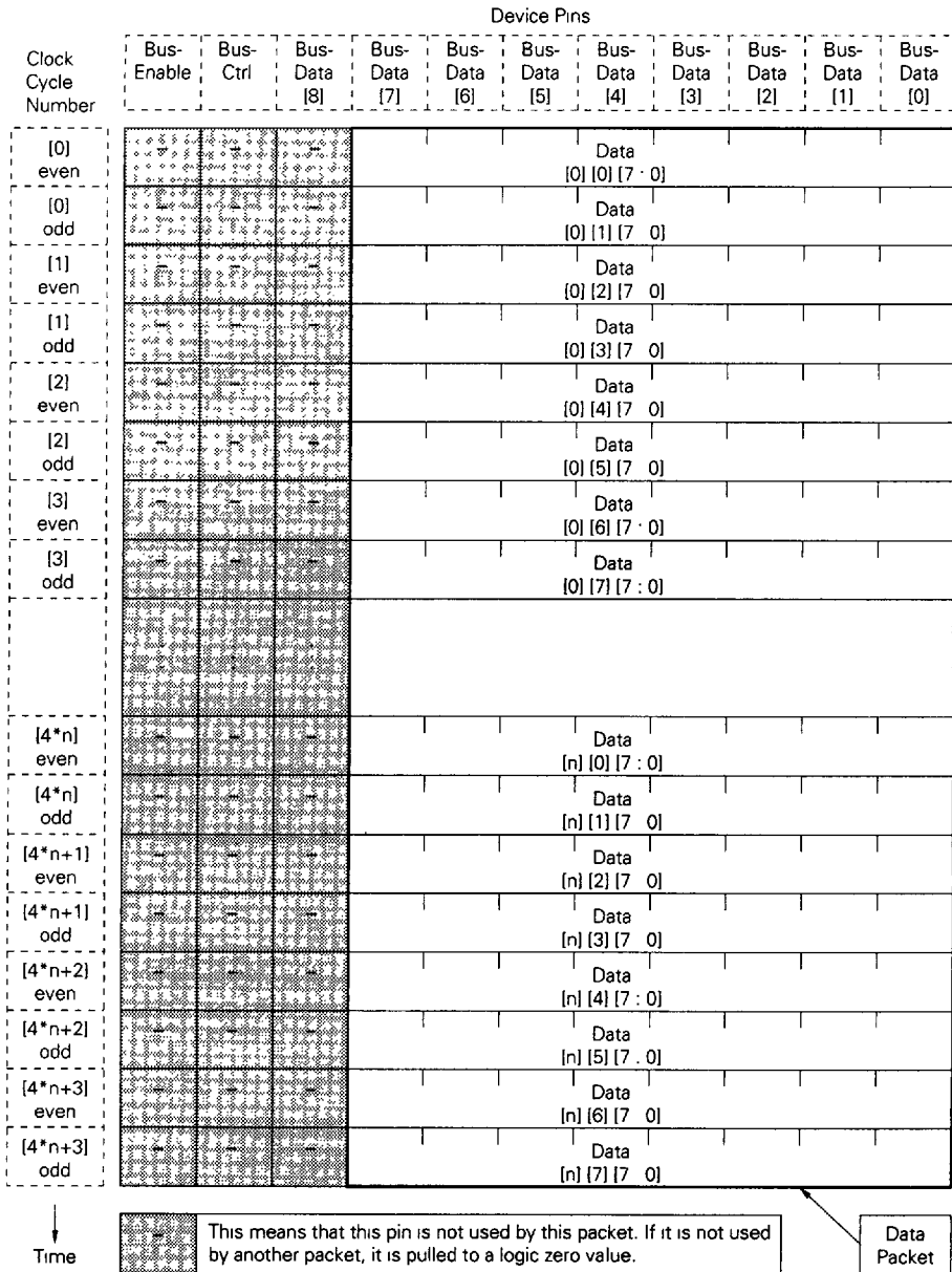
Figure 5-4. Data Packet Format (Memory Space)
