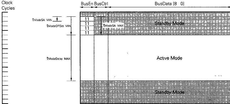
Figure 6-3. Basic ActiveMode/StandbyMode Transitions
