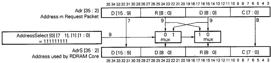
Figure 9-1. AddressMapping Hardware
