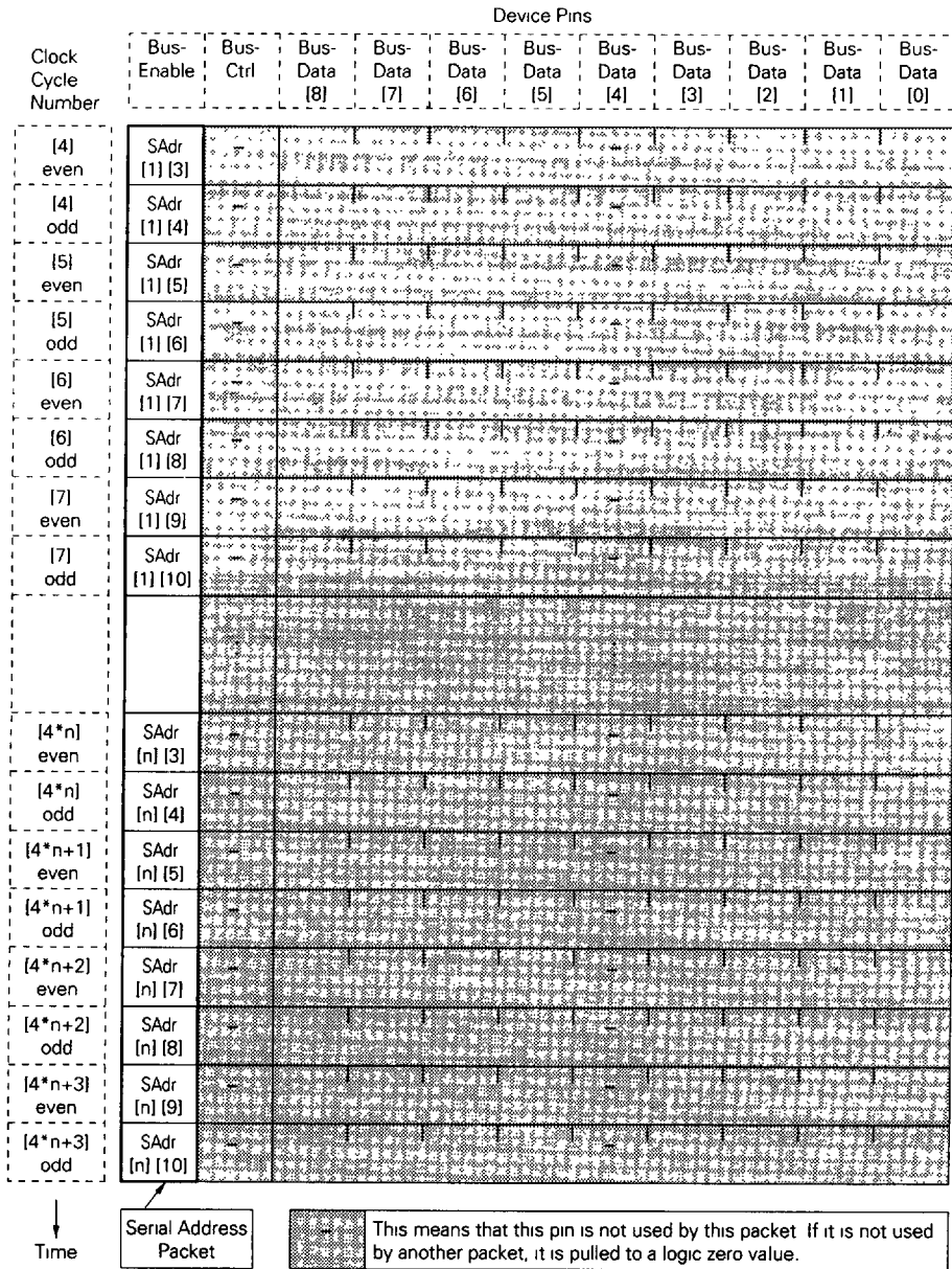
Figure 5-5. Serial Address Packet Format
