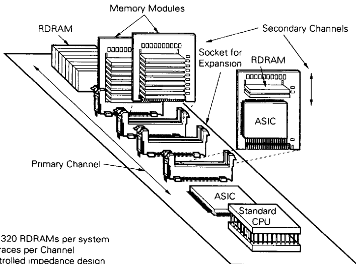
Figure 2-2. A Rambus System Example
