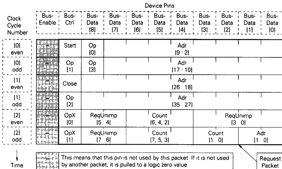
Figure 5-1. Request Packet Format
