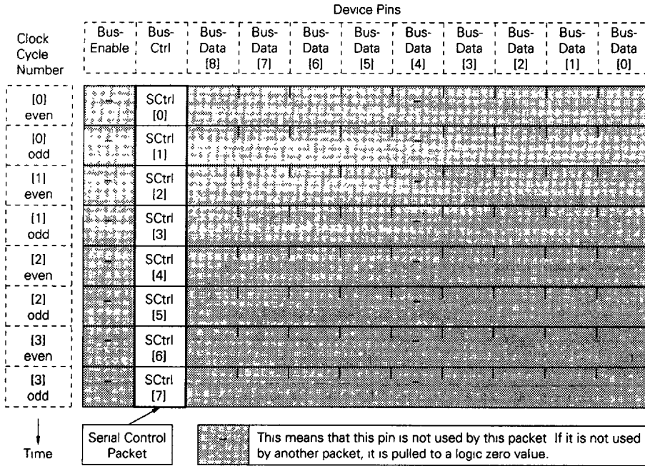
Figure 5-6. Serial Control Packet Format
