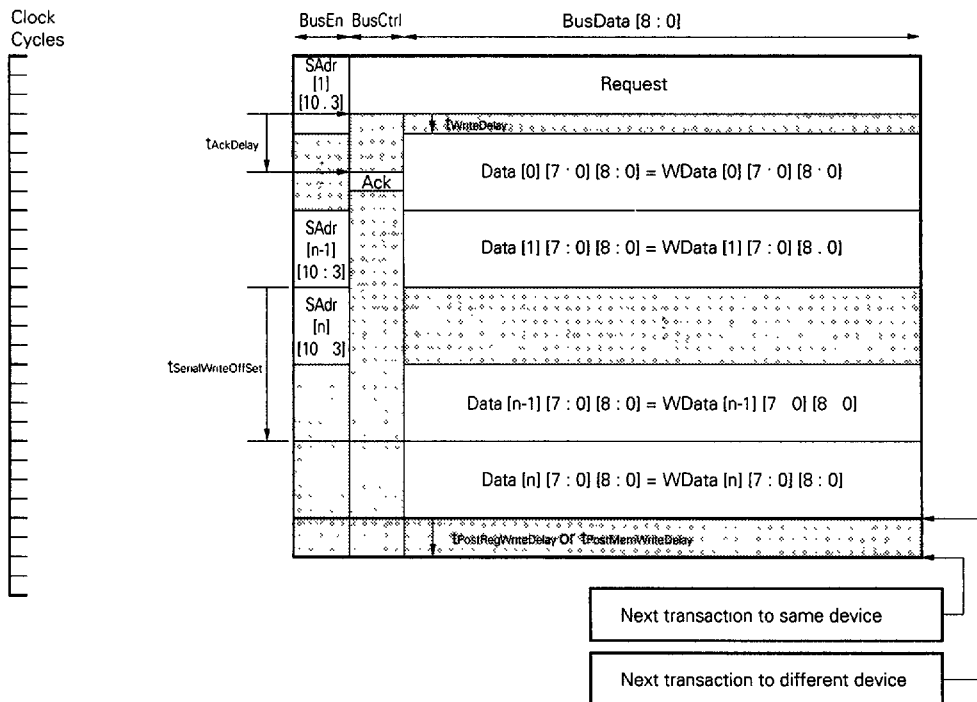
Figure 7-4. Write Transaction with Serial Address Packet
