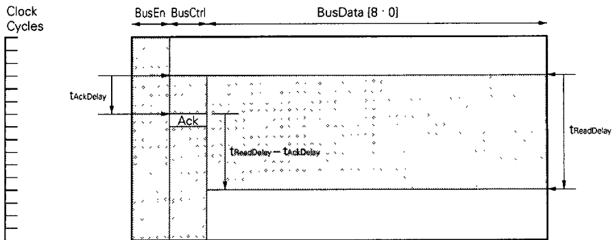
Figure 7-1. Read Transaction
