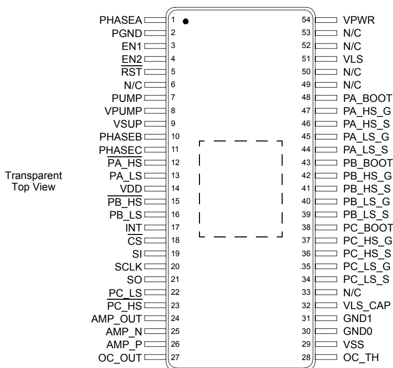
Figure 3. 33937 Pin Connections
