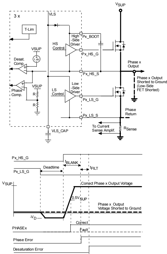
Figure 18. Short to Ground Detection
