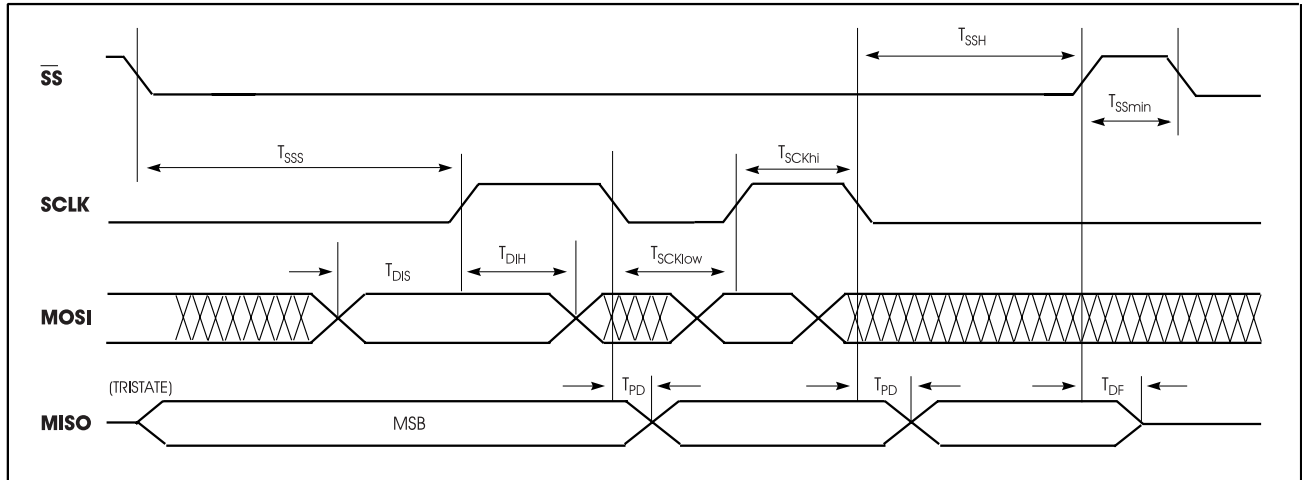
Figure 6: Timing Diagram
