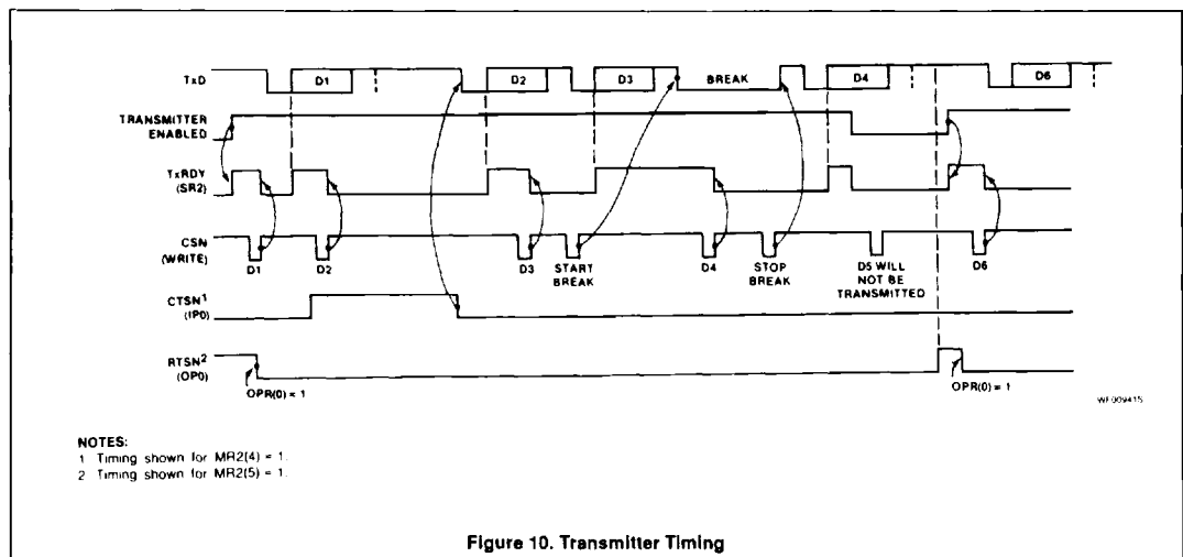
Figure 10. Transmitter Timing
