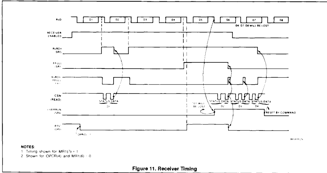
Figure 11. Receiver Timing
