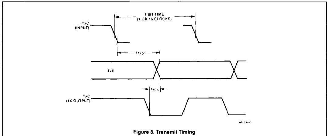
Figure 8. Transmit Timing
