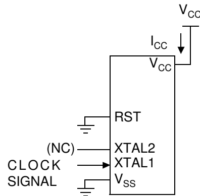
Figure 1. I_{CC} Test Condition, Under Reset
