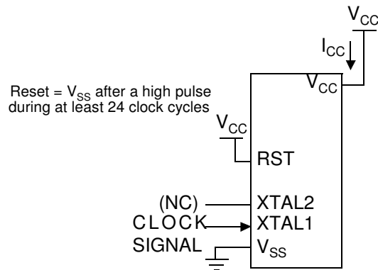
Figure 2. Operating I_{CC} Test Condition
