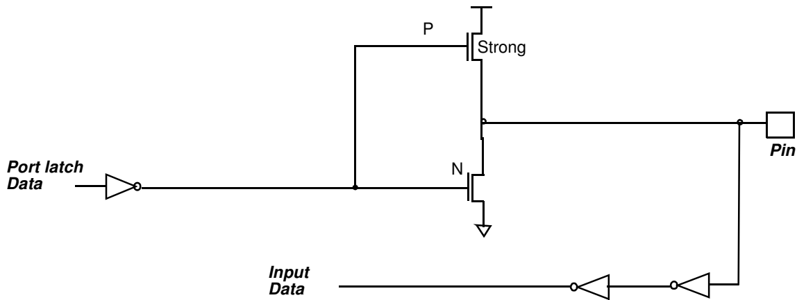
Figure 3. Push-pull Output
