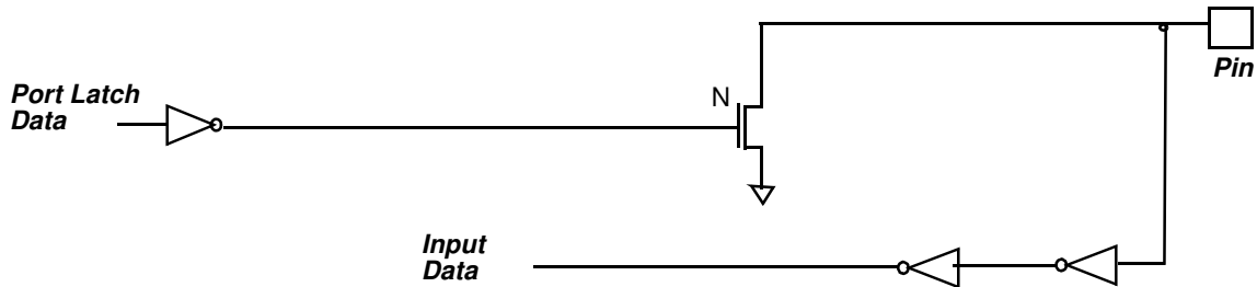
Figure 2. Open-drain Output
