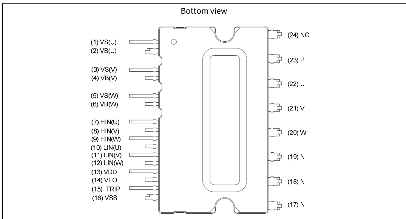
Figure 2 Pin configuration
