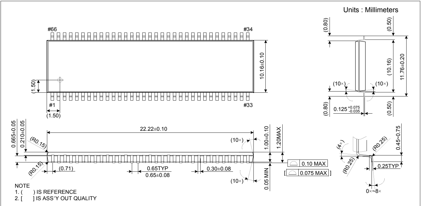
66pin TSOP II / Package dimension
