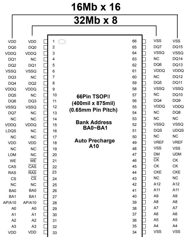
512Mb TSOP-II Package Pinout
