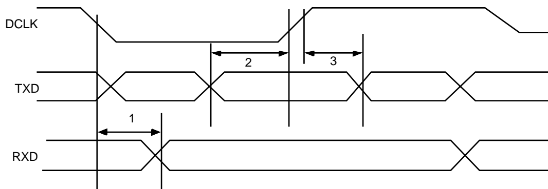
Figure 5. Serial Port Timing Diagram
