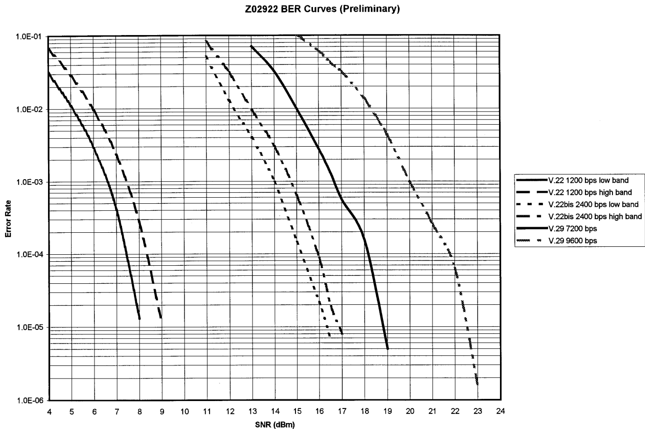
Figure 9. Typical Performance Data
