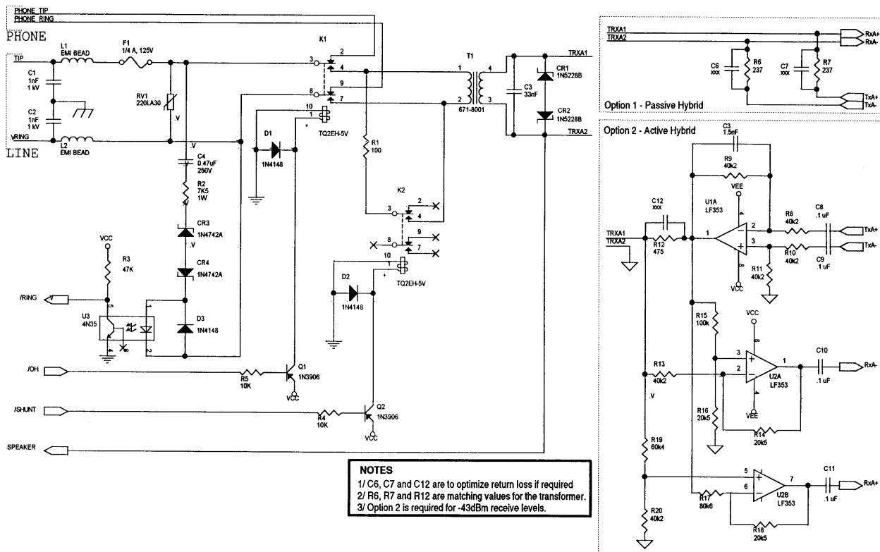
Figure 11. Example DAA
