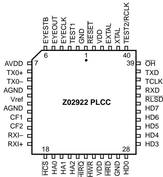
Figure 3. Z02922 44-Lead PLCC Pin Identification
