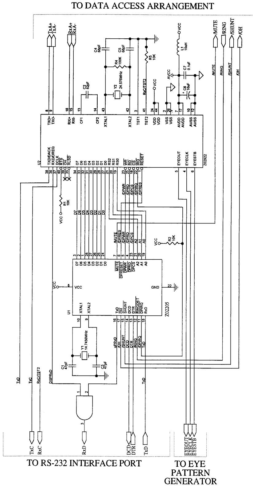
Figure 10. Typical Modem Using Z02922
