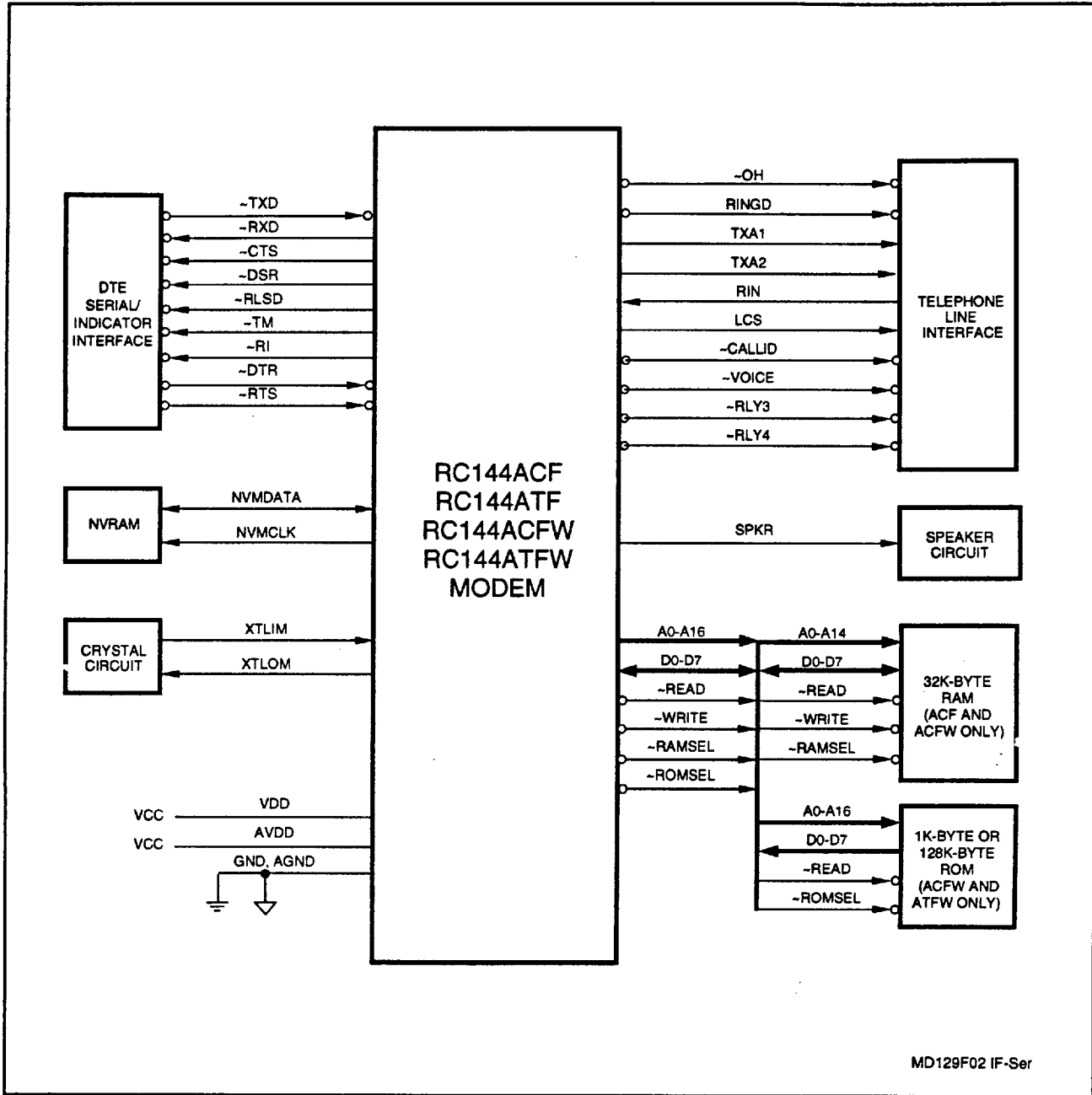
Figure 2. Hardware Interface Signals - Serial Interface
