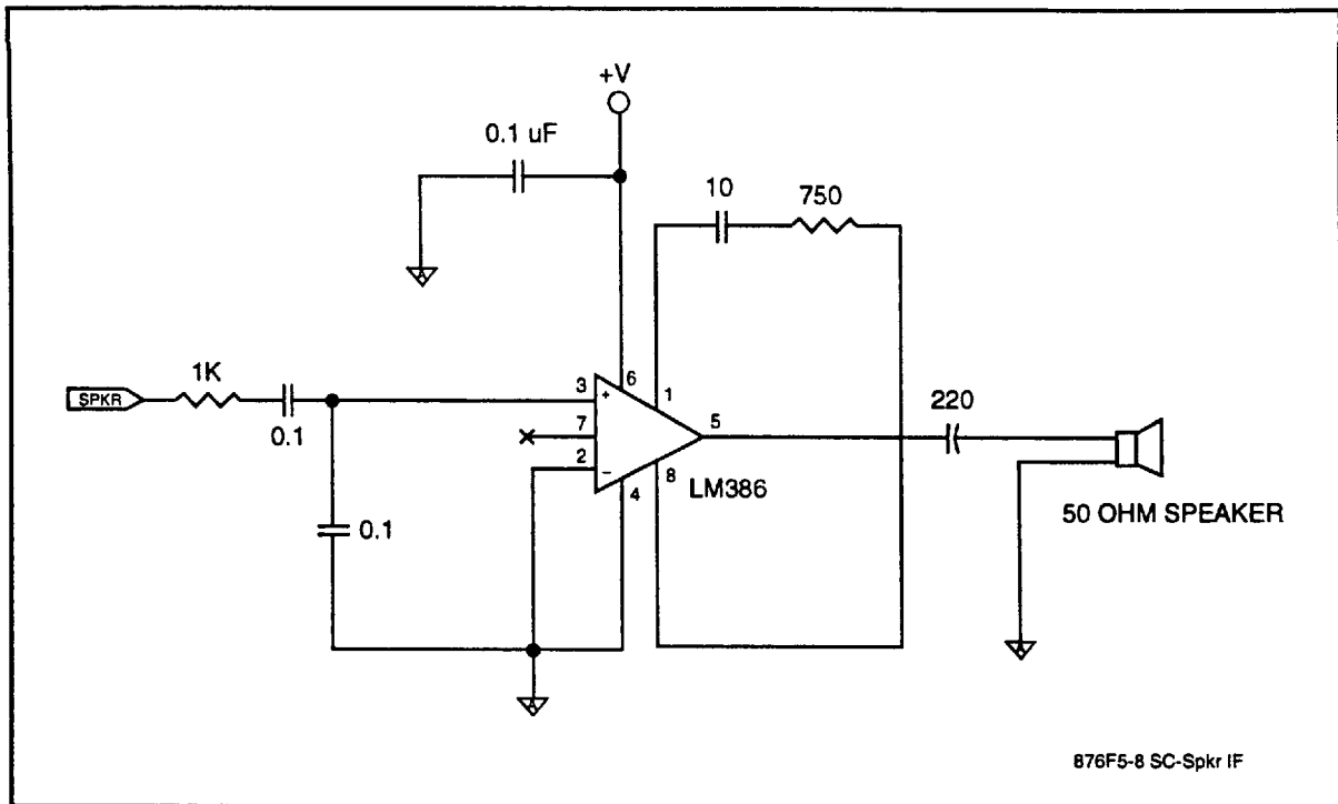
Figure 10. Typical External Speaker Circuit
