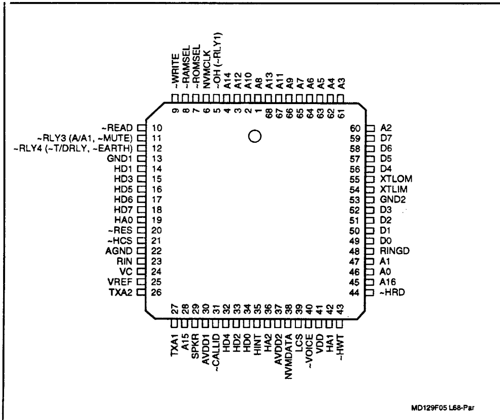
Figure 5. Pin Signals - 68-Pin PLCC - Parallel Interface
