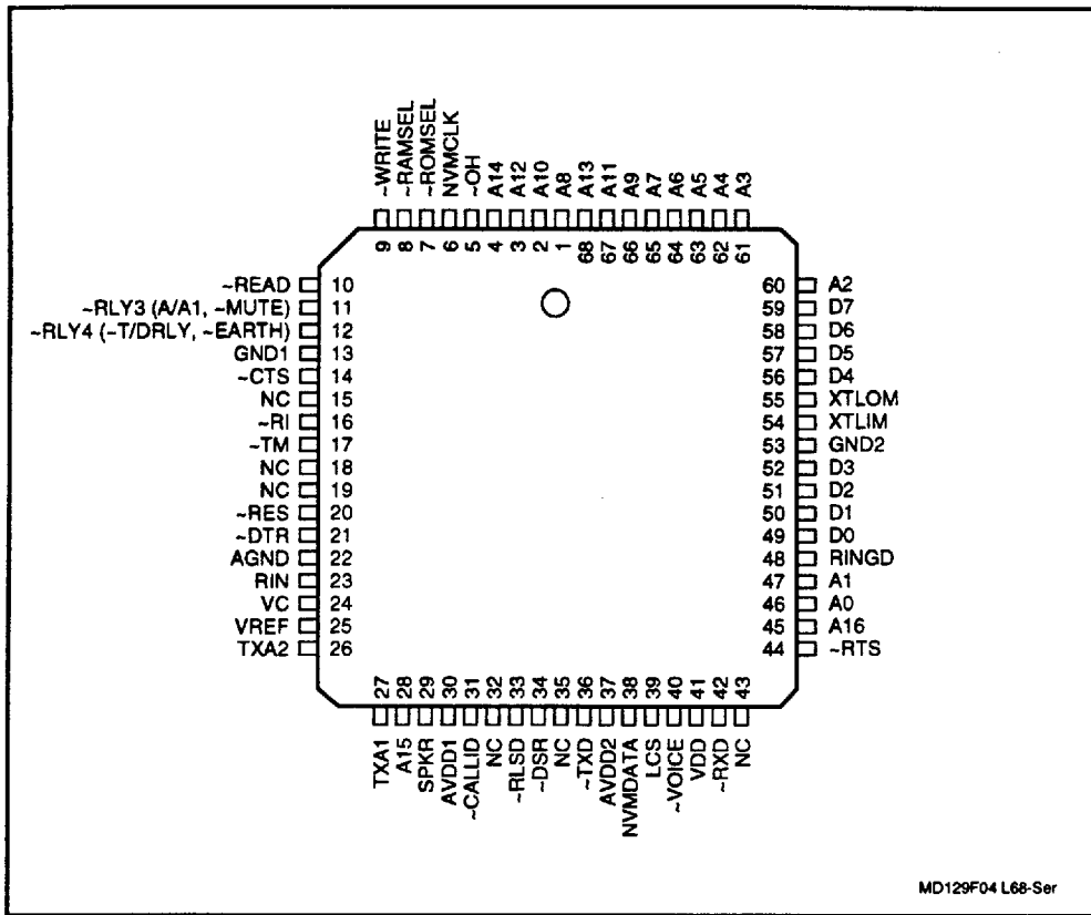
Figure 4. Pin Signals - 68-Pin PLCC - Serial Interface
