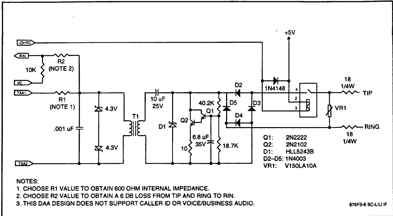
Figure 8. Typical Line Interface
