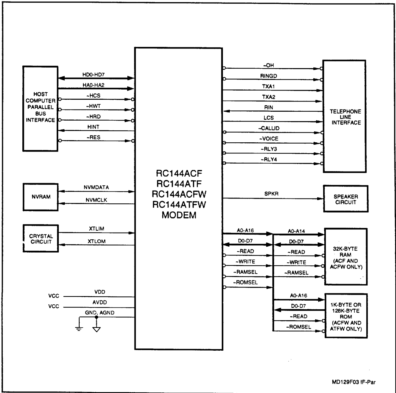
Figure 3. Hardware Interface Signals - Parallel Interface
