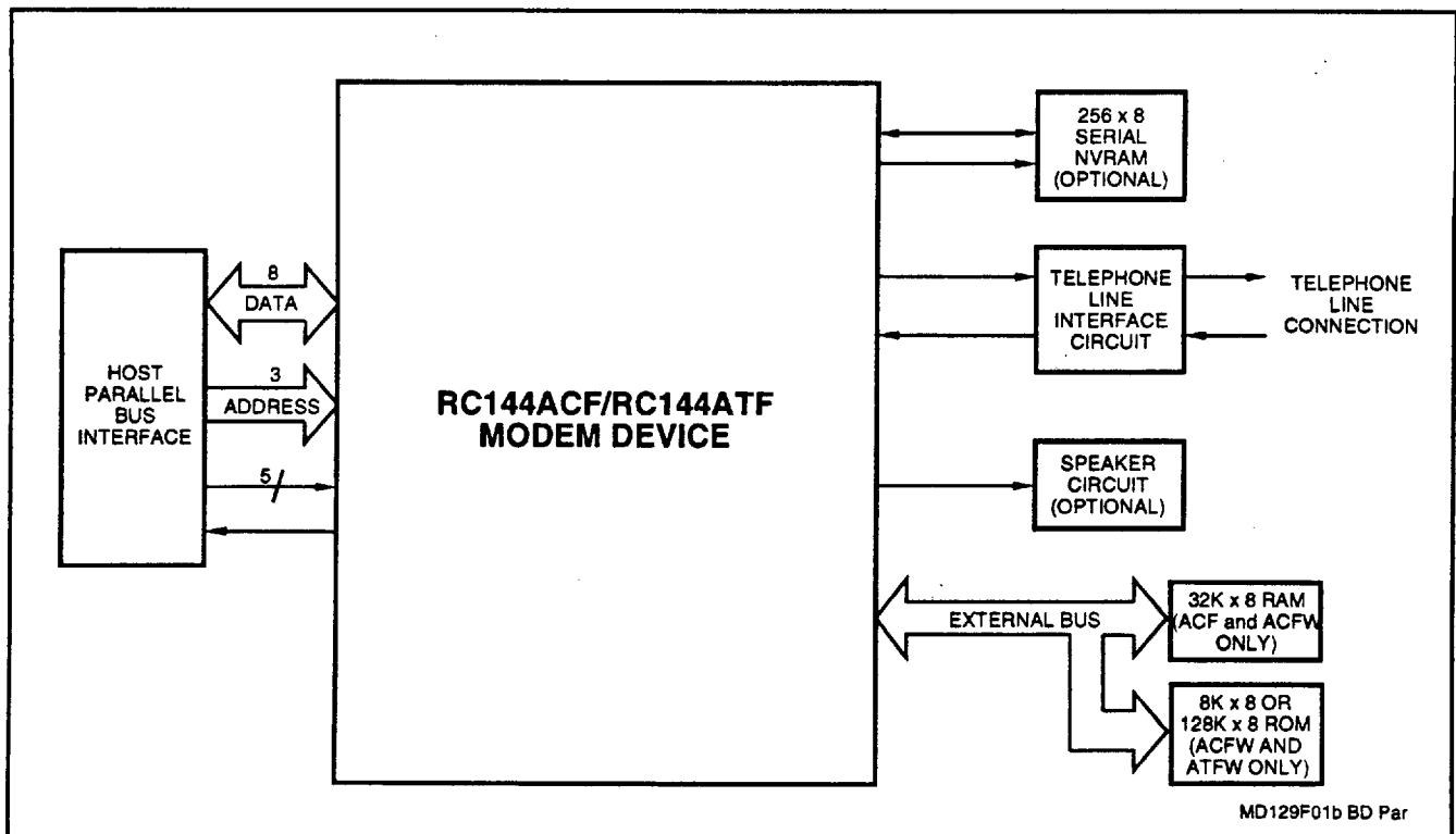
Figure 1b. Block Diagram - Parallel Interface
