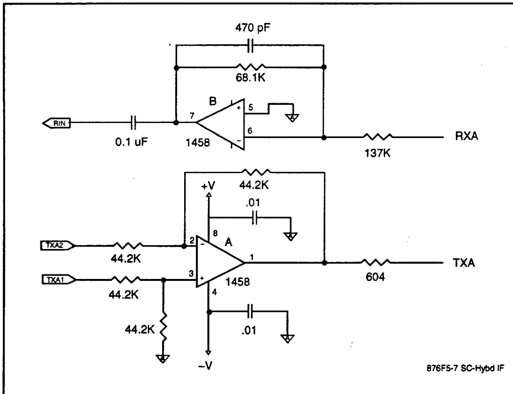
Figure 9. Typical Interface to External Hybrid
