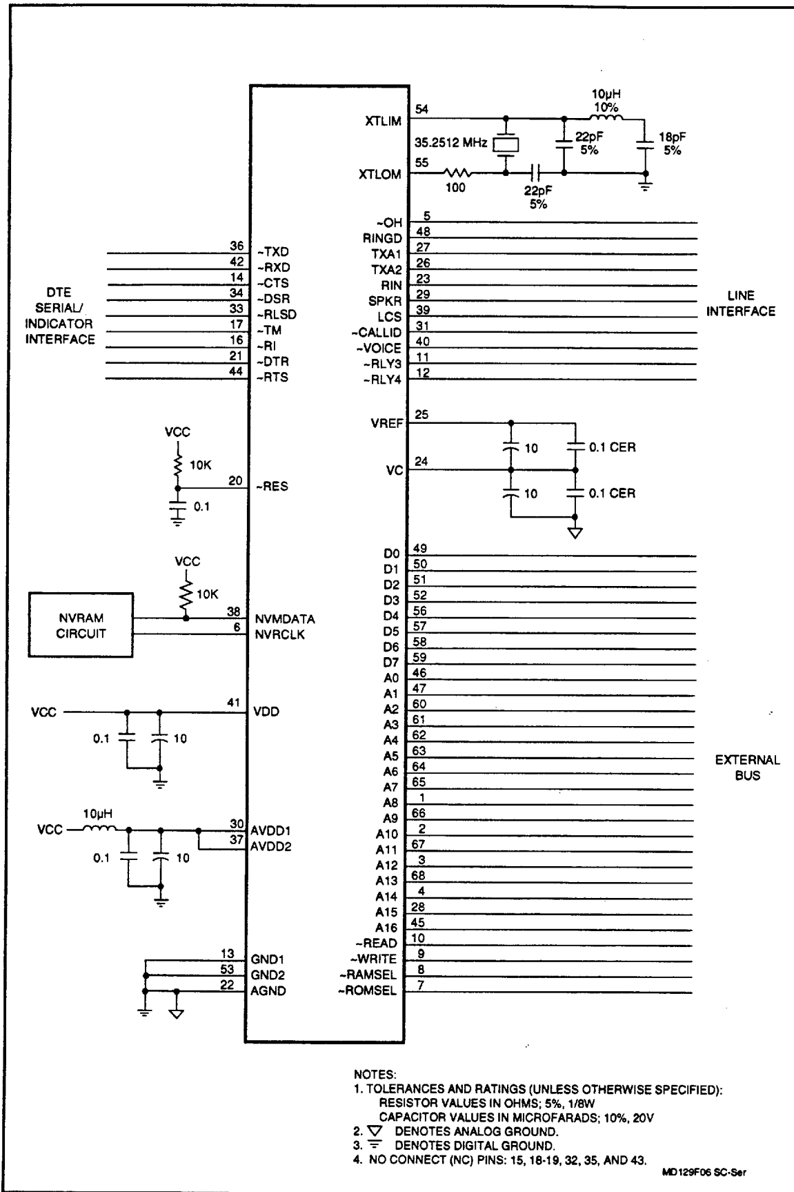
Figure 6. Interface Schematic - Serial DTE Interface
