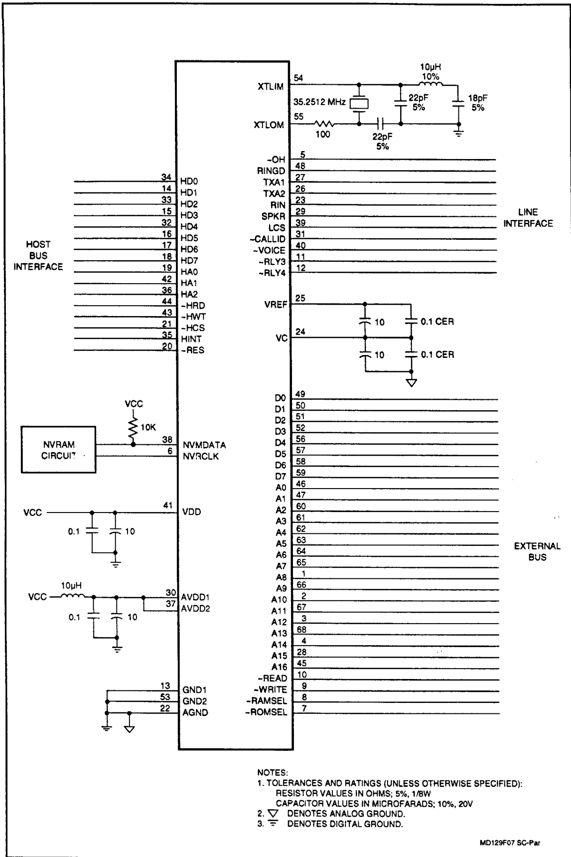
Figure 7. Interface Schematic - Parallel Host Interface
