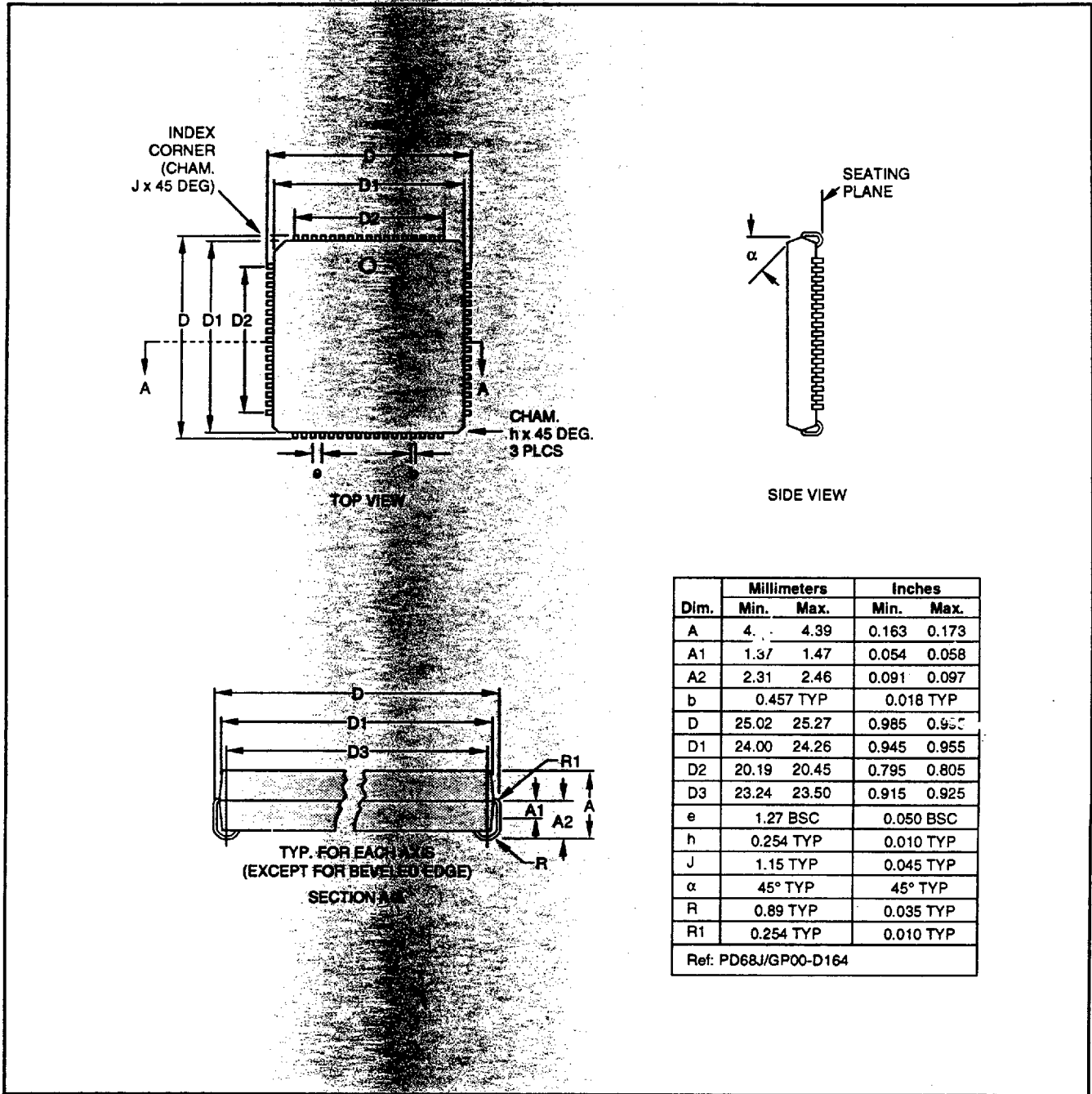
Figure 11. Package Dimensions - 68-Pin PLCC
