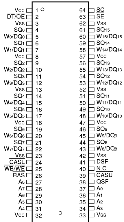
64-Pin 525 mil SSOP
