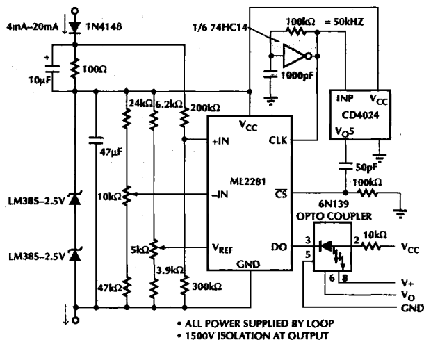
4mA-20mA Current Loop Converter
