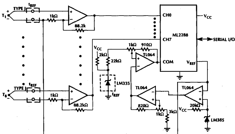
Convert 8 Thermocouples with only One Cold-Junction Compensator
