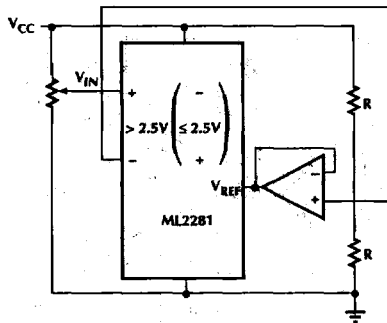
Obtaining 9-Bit Resolution
