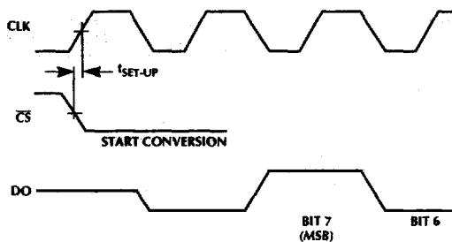
Figure 2. Timing Diagrams
