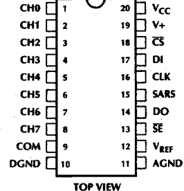
ML2288 8-Channel MUX 20-Pin DIP
