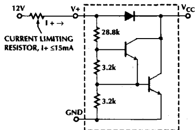
Figure 8. Shunt Regulator
