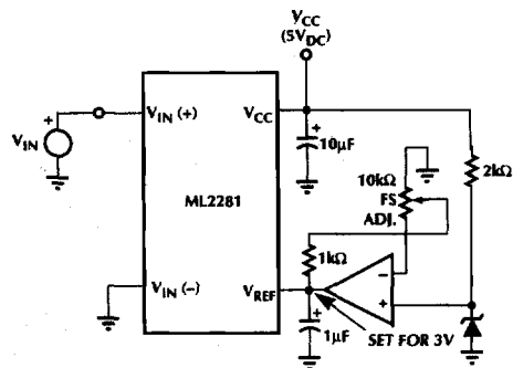
Digitizing a Current Flow
