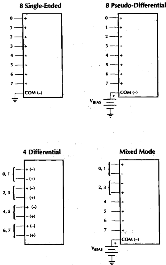
Figure 7. Analog Input Multiplexer Functional Options for ML2288
