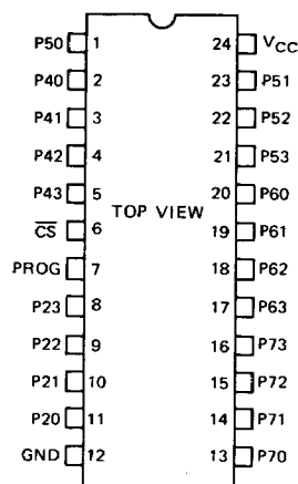
Fig. 1 — PIN ASSIGNMENT
