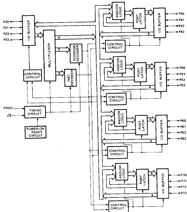
Fig. 3 – BLOCK DIAGRAM
