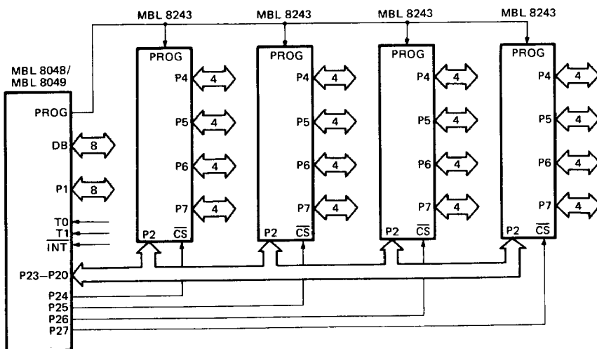
Fig. 6 – MULTIPLE I/O EXPANDER INTERFACE
