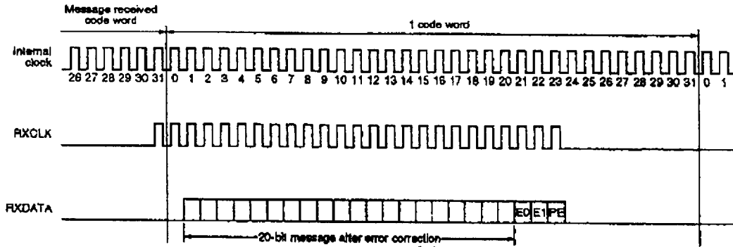
Figure 11. Received message transfer timing
