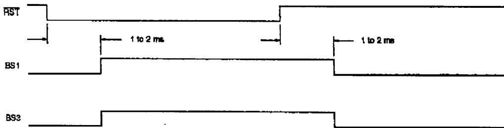
Figure 13. Reset timing
