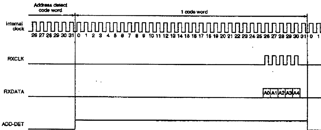
Figure 10. Received address data timing
