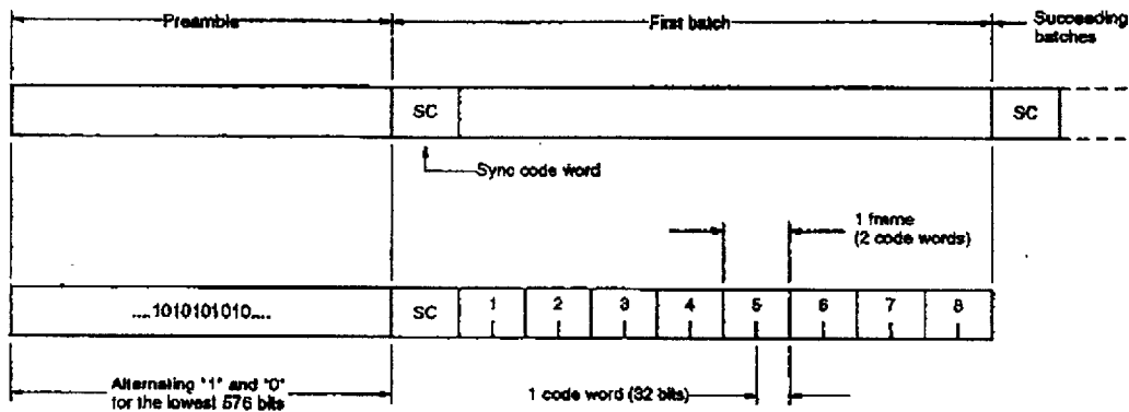
Figure 4. Data format
