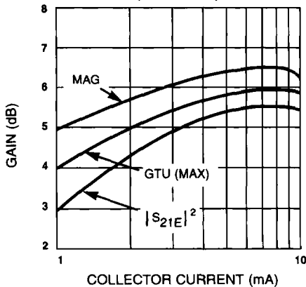
GAIN vs COLLECTOR CURRENT AT 3 GHz AND V_{CE} = 3V (MA4T631035)
