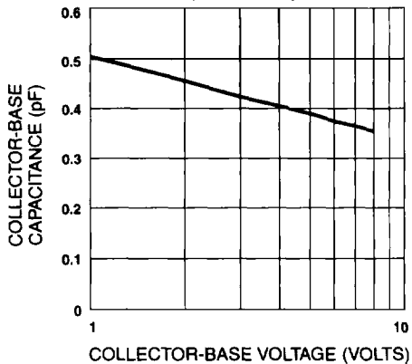
COLLECTOR-BASE CAPACITANCE ( C_{OB} ) vs COLLECTOR-BASE VOLTAGE (MA4T631035)
