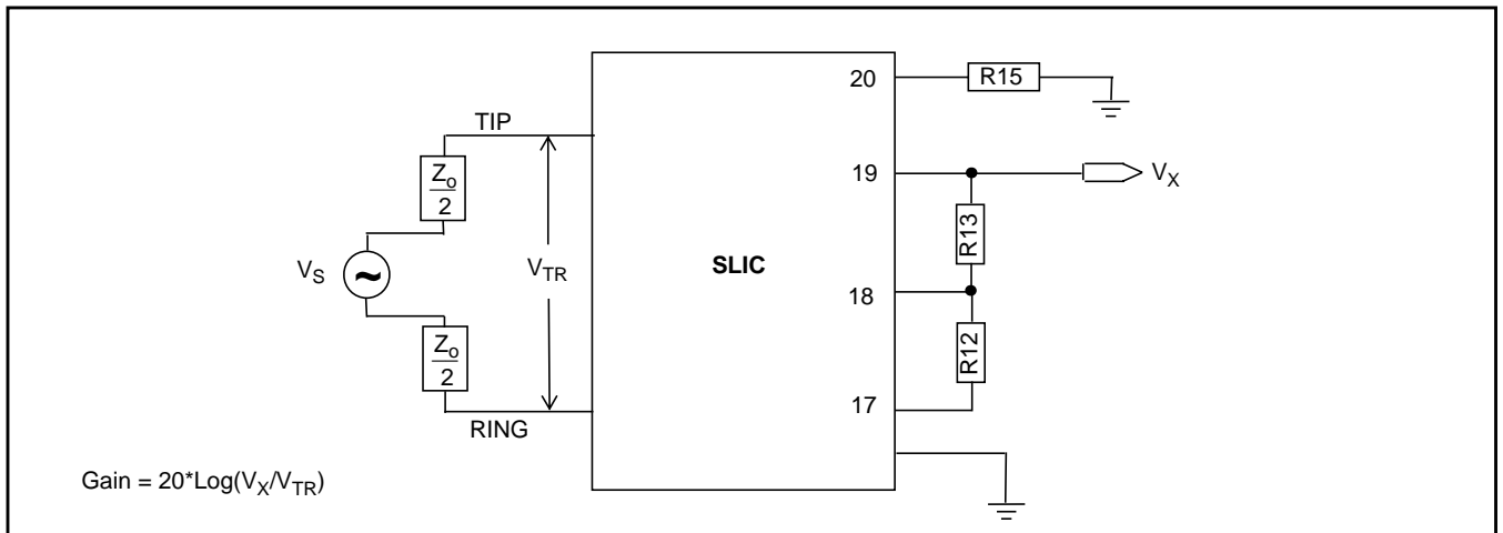
Figure 7 - 2-4 Wire Gain
