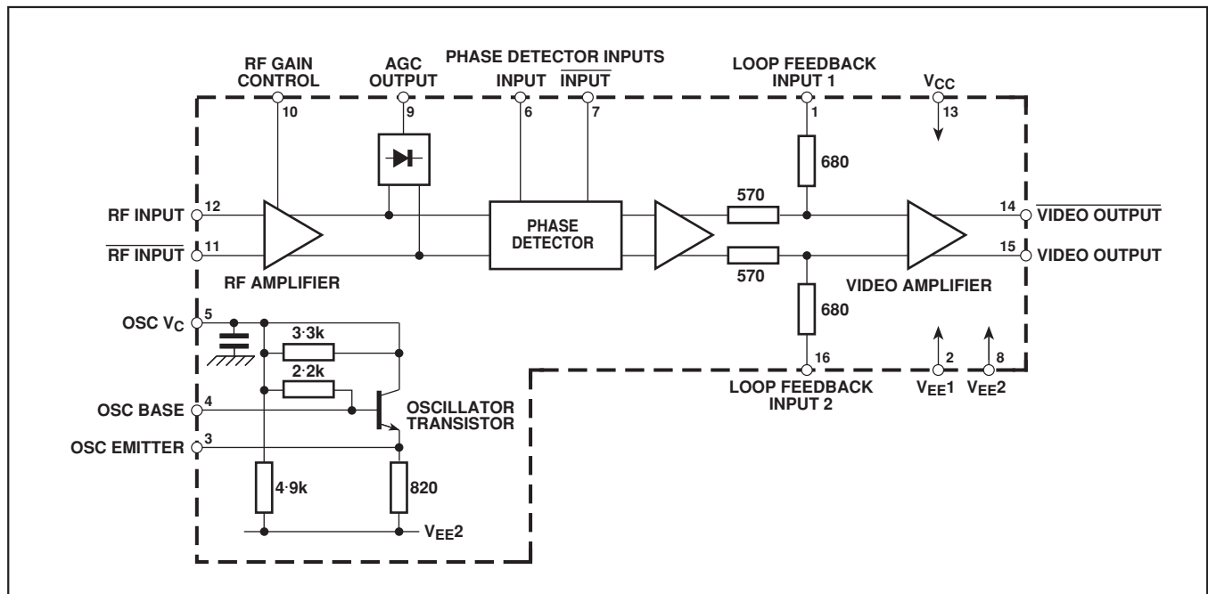
Fig. 2 Block diagram
