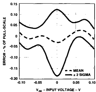
Figure 13. 100 mV Nonlinearity Error Plot.
