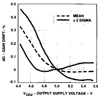
Figure 8. Gain Drift vs. V_{DD2} ( V_{DD1} = 5\text{ V} ).
