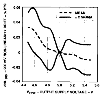
Figure 12. 200 mV Nonlinearity Drift vs. V_{DD2} ( V_{DD1} = 5 V).
