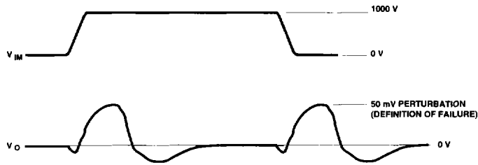
Figure 20. Typical IMR Failure Waveform.
