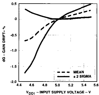
Figure 7. Gain Drift vs. V_{DD1} ( V_{DD2} = 5\text{ V} ).
