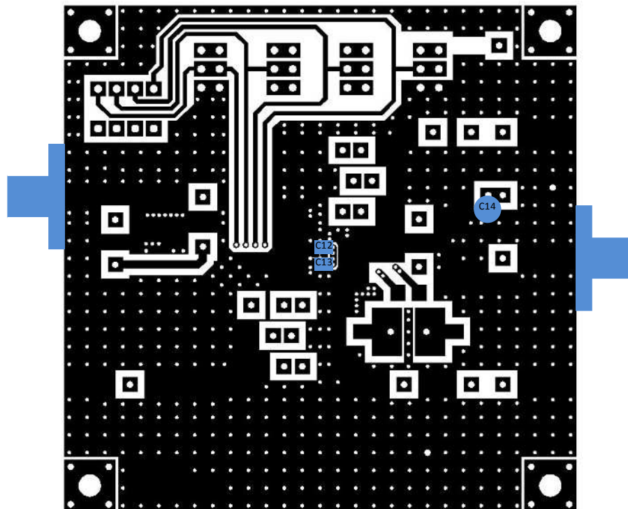
Bottom View
