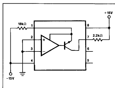
BURN-IN CIRCUIT
