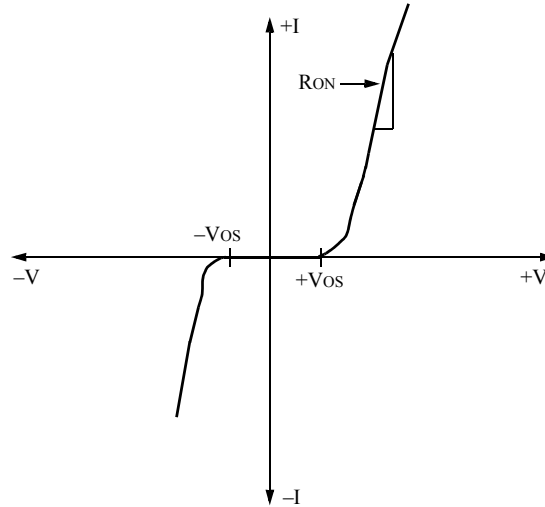
Figure 5. Switches 6, 8
