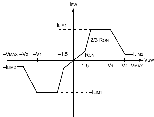
Figure 4. Switches 1, 2, and 5
