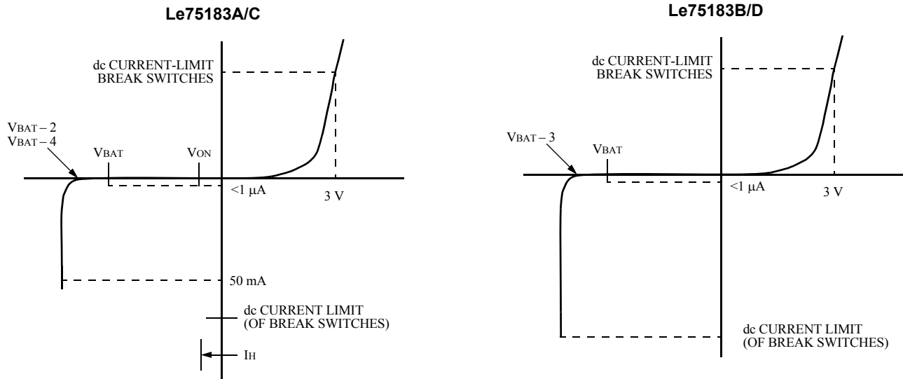
Figure 1. Protection Circuits
