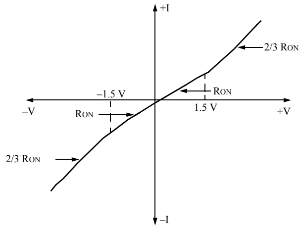
Figure 4. Switches 1, 2, and 5
