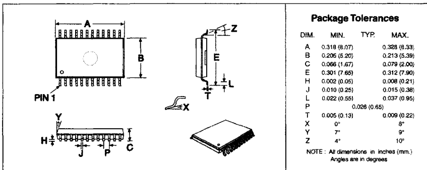
Figure 27: 24-pin SSOP Mechanical Outline : Order as part no. MX929ADS
