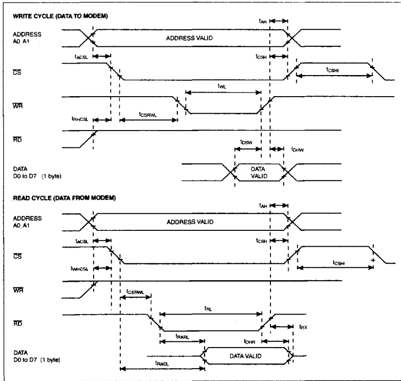
Figure 24: \mu C Parallel interface Timings
