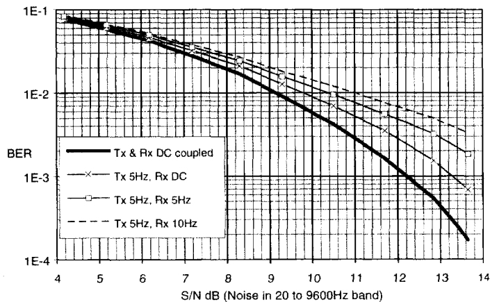
Figure 21: Effect of AC Coupling on BER
