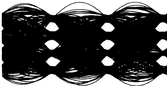
Figure 6: Transmitted Signal Eye Diagram
