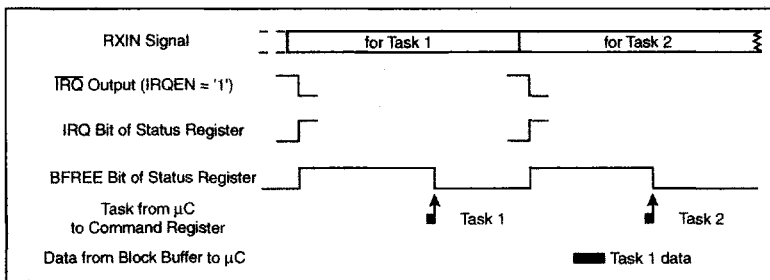
Figure 10: Receive Task Overlapping
