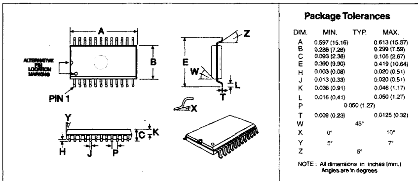
Figure 26: 24-pin SOIC Mechanical Outline : Order as part no. MX929ADW
