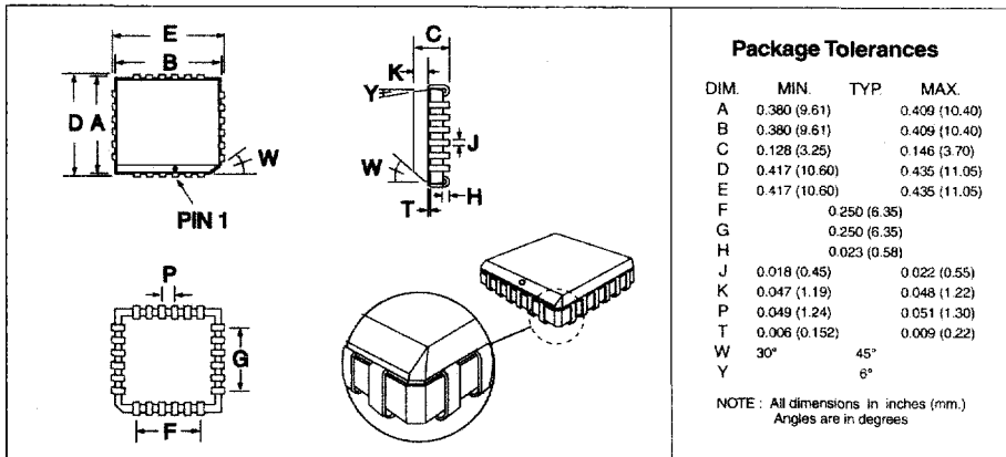
Figure 28: 24-pin PLCC Mechanical Outline : Order as part no. MX929ALH
