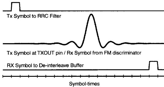
Figure 13: RRC Low Pass Filter Delay
