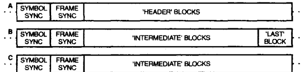
Figure 8: Some Alternative Frame Structures
