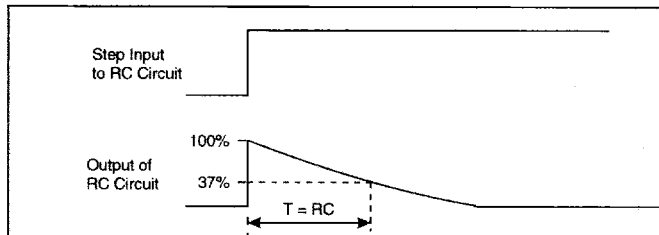
Figure 22: Decay Time - AC Coupling
