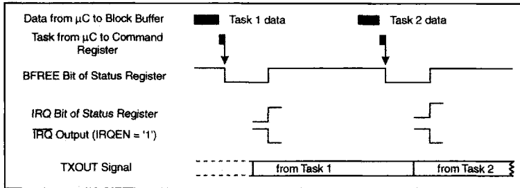
Figure 9: Transmit Task Overlapping
