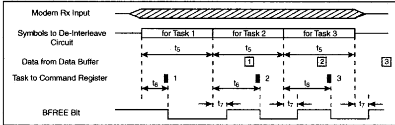
Figure 12: Receive Task Timing Diagram
