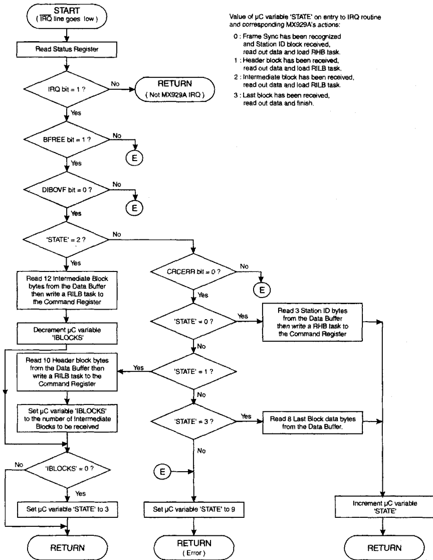
Figure 19: Receive Interrupt Service Routine
