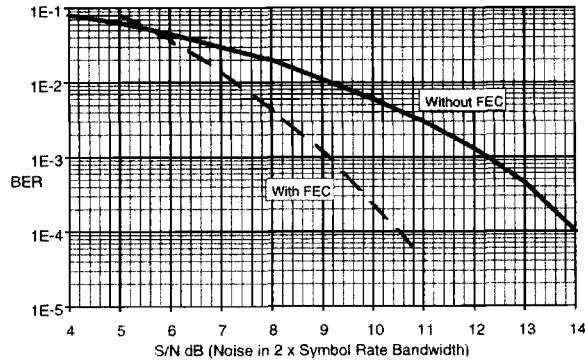
Figure 25: Typical Bit Error Rate With and Without FEC
