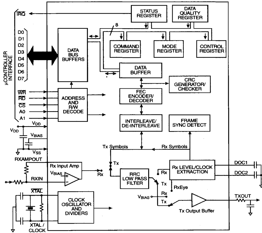
Figure 1: Block Diagram
