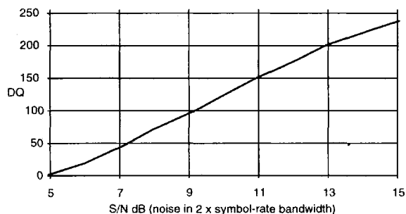
Figure 15: Typical Data Quality Reading vs S/N
