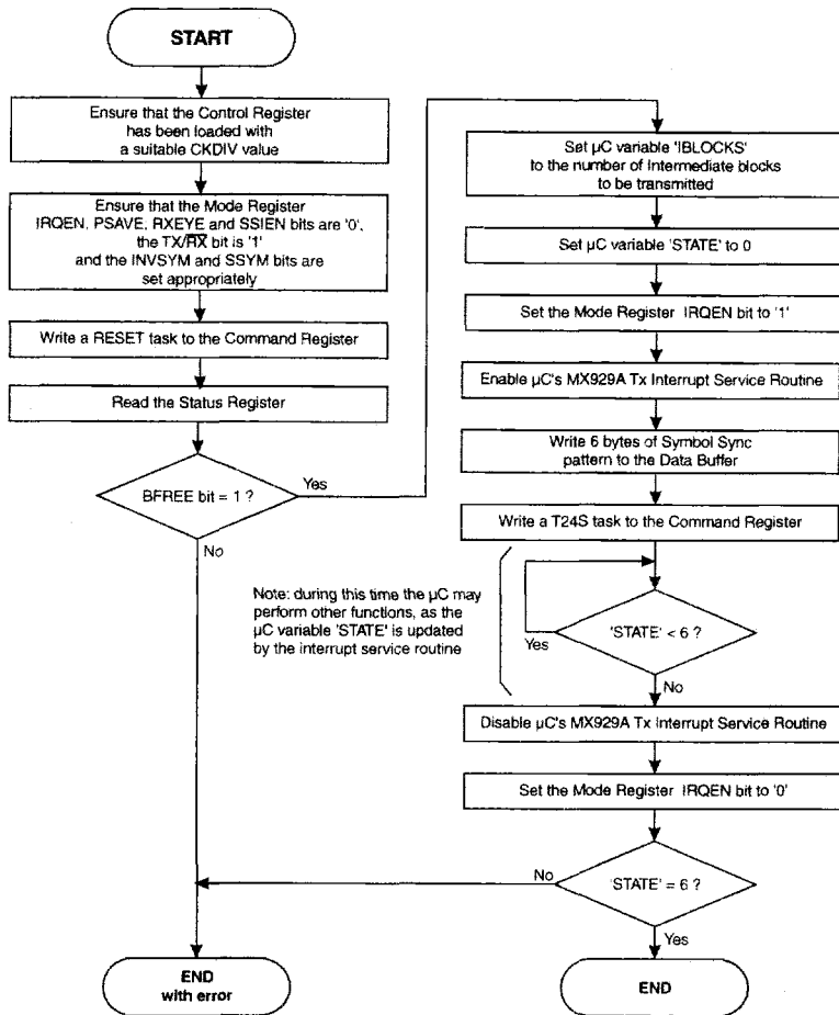
Figure 16: Transmit Frame Example Flowchart , Main Program
