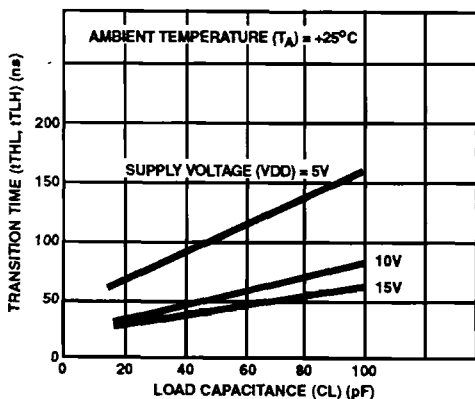
FIGURE 13. TYPICAL TRANSITION TIME AS A FUNCTION OF LOAD CAPACITANCE
