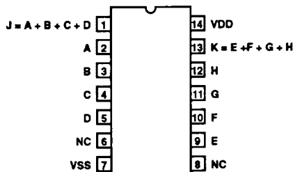
CD4072BMS TOP VIEW
