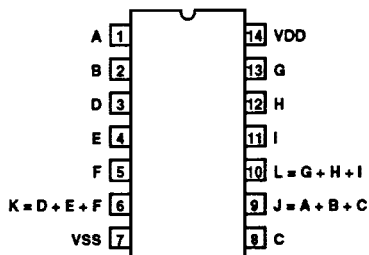
CD4075BMS TOP VIEW
