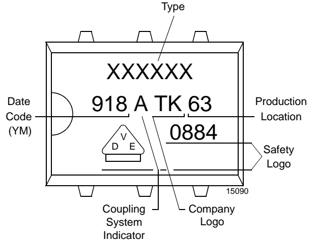
Figure 13. Marking example
