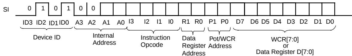
Figure 9. Increment/Decrement Instruction Sequence
