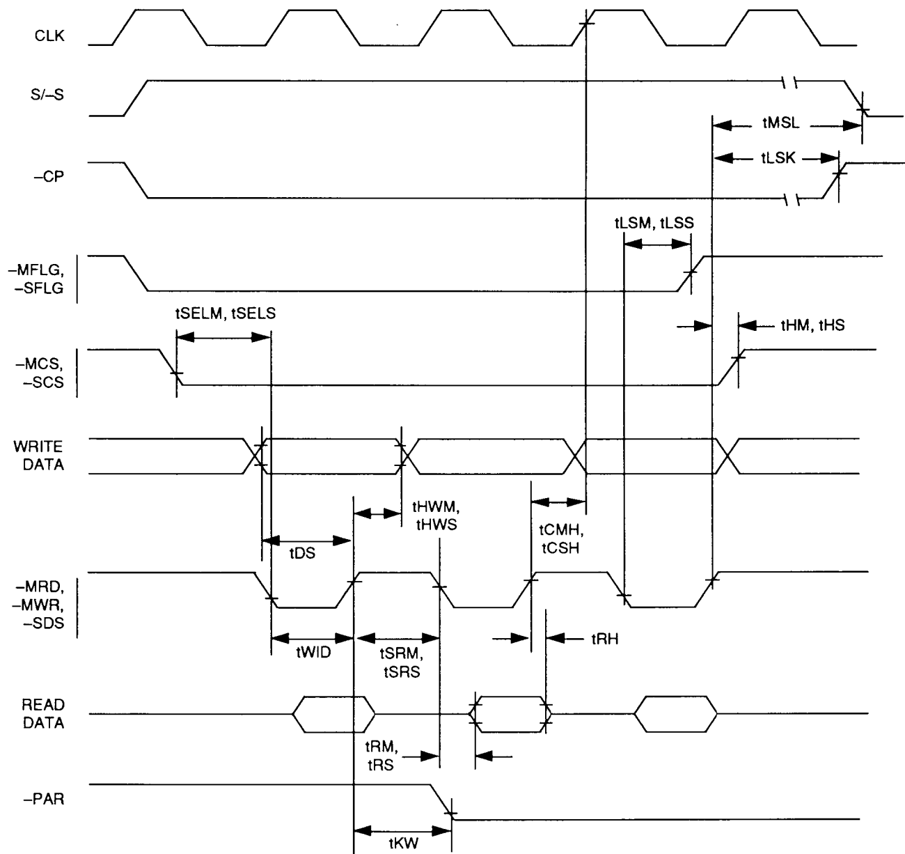
FIGURE 12. MASTER (SLAVE) PORT READ/WRITE (VM009-A-86)
