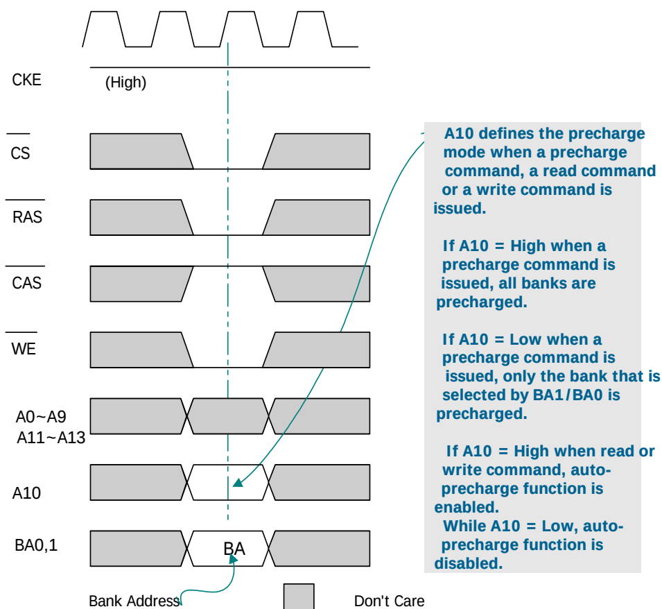
PRECHARGE command
