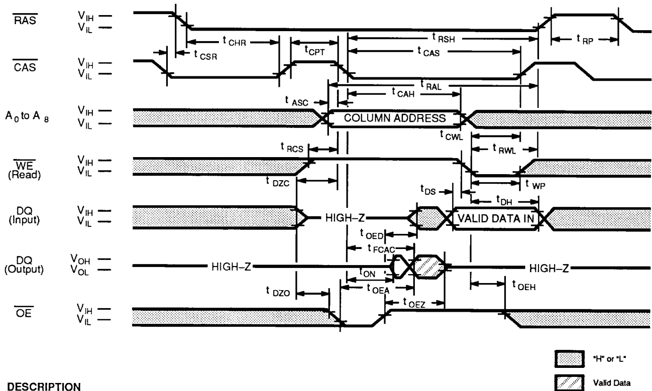
Fig. 15 – \overline{\text{CAS}} -BEFORE- \overline{\text{RAS}} REFRESH COUNTER TEST CYCLE
