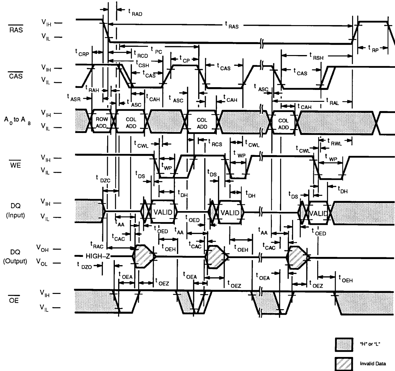
Fig. 10 – FAST PAGE MODE \overline{OE} WRITE CYCLE
