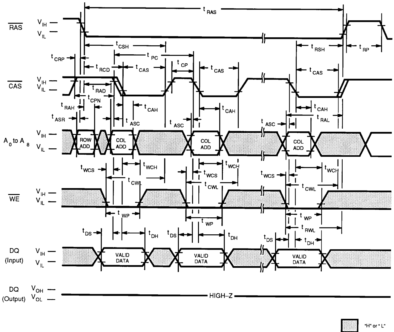
Fig. 9 – FAST PAGE MODE WRITE CYCLE ( \overline{OE} = \text{"H" or "L"} )
