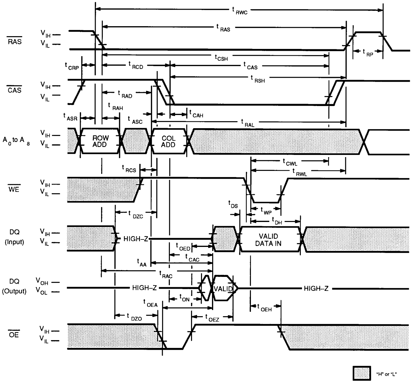
Fig. 7 - READ-MODIFY-WRITE CYCLE
