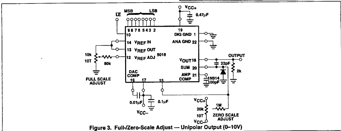
Figure 3. Full/Zero-Scale Adjust — Unipolar Output (0-10V)
