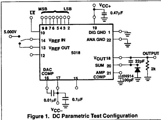
Figure 1. DC Parametric Test Configuration
