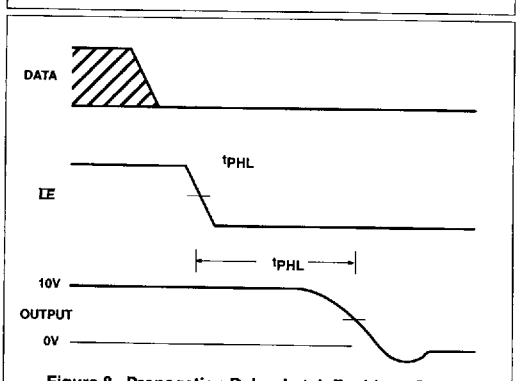
Figure 8. Propagation Delay, Latch Enable to Output
