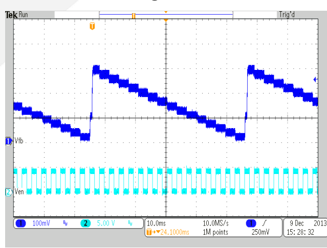
Dimming waveform
