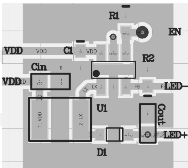
Figure 8. PCB Layout recommended
