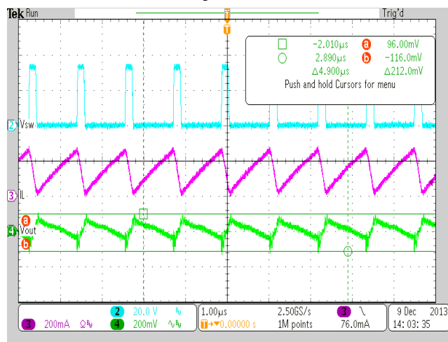
Stability waveform
