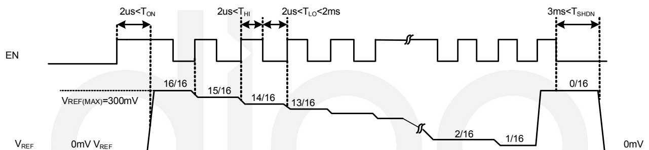
Figure 5. Timing of Pin EN
