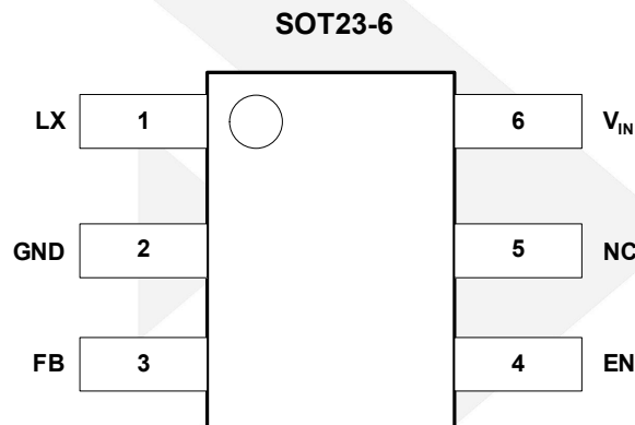
Figure 1 Top View
