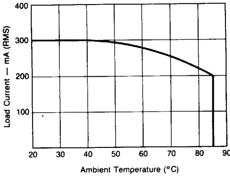
Figure 1. Derating Curve
