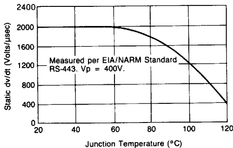
Figure 4. Typical Static dv/dt Performance
