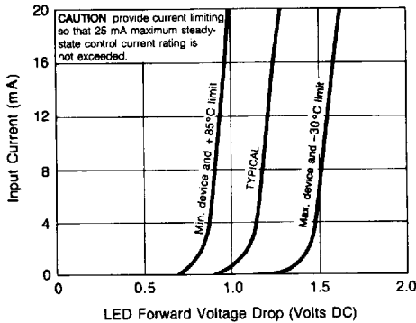
Figure 3. Input Characteristics (Current Controlled)
