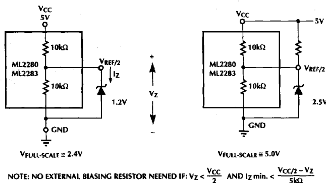
Figure 8. Reference Biasing
