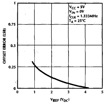
Figure 5. Unadjusted Offset Error vs V_{REF} Voltage
