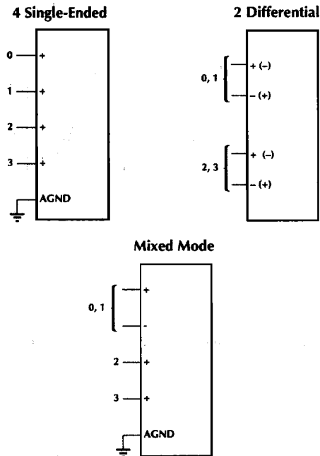
Figure 7. Analog Input Multiplexer Functional Options for ML2288
