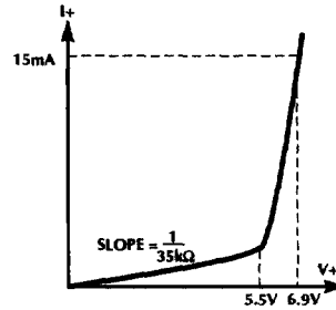
Figure 10. I-V Characteristic of the Shunt Regulator
