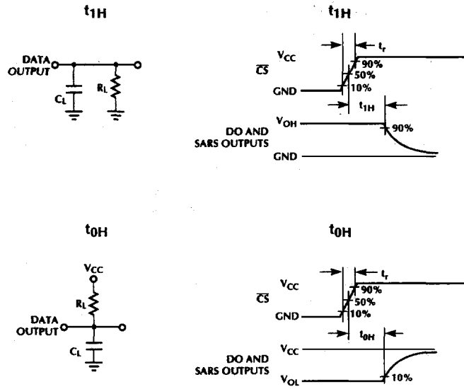
Figure 1. High Impedance Test Circuits and Waveforms
