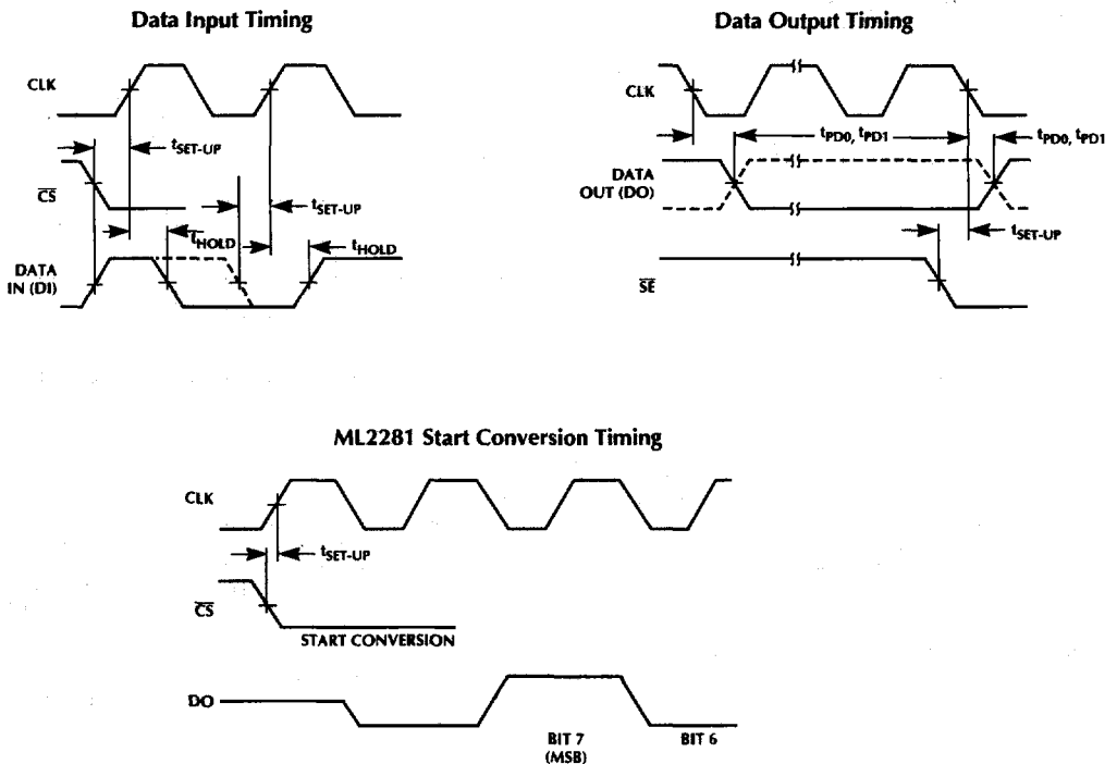
Figure 2. Timing Diagrams
