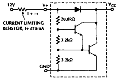
Figure 9. Shunt Regulator
