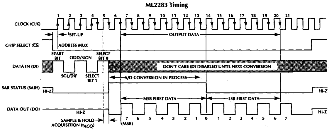
Figure 2. Timing Diagrams (Continued)
