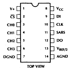
ML2283 4-Channel MUX 14-Pin PDIP
