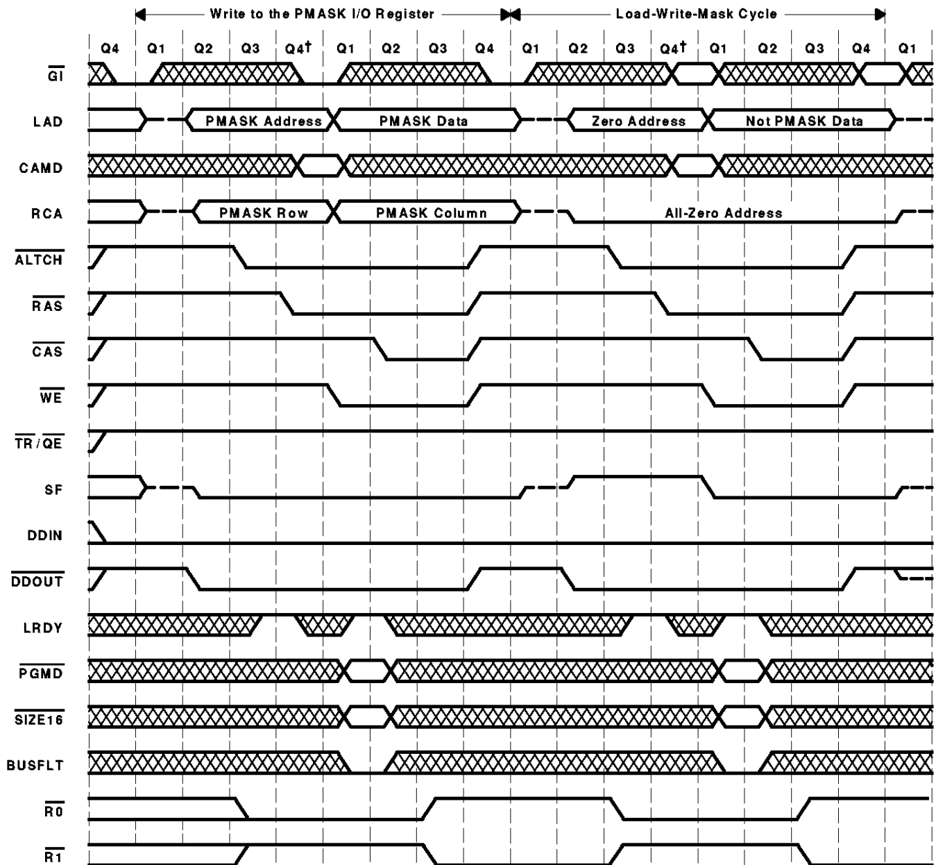
Figure 9. Load-Write-Mask-Cycle Timing
