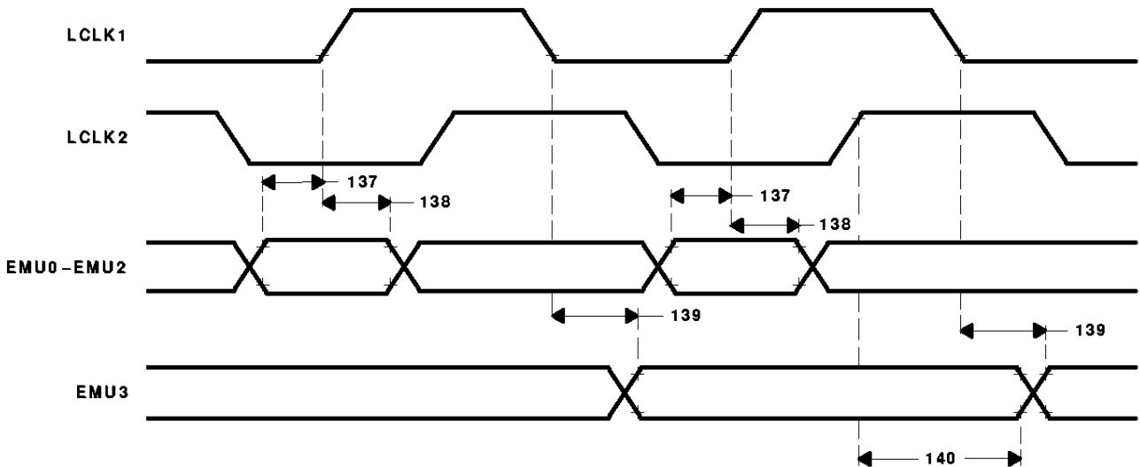
Figure 51. Emulator-Interface Timing
