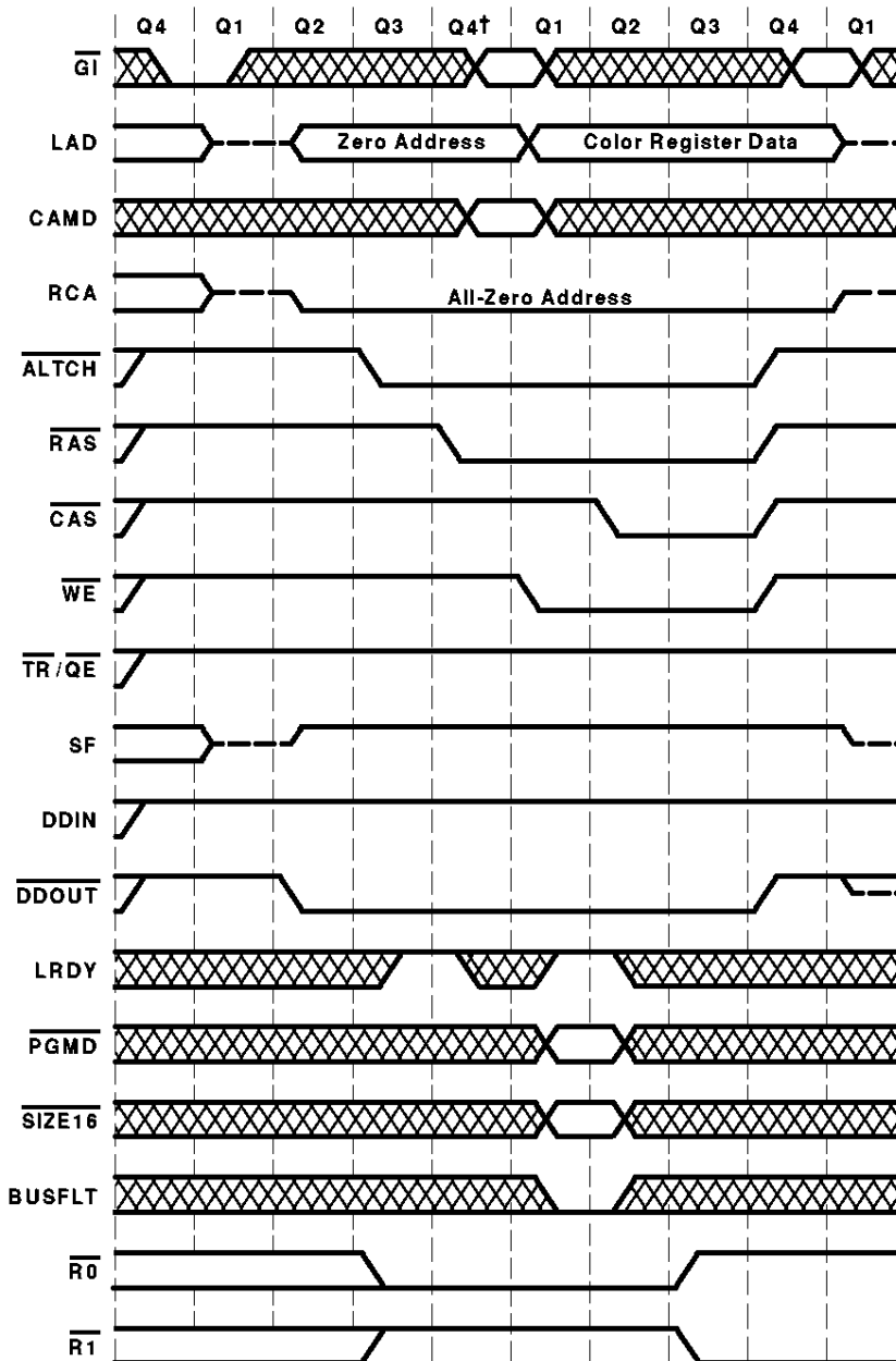
Figure 10. Load-Color-Latch-Cycle Timing
