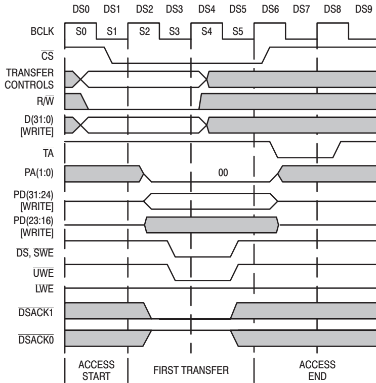
Figure 42. 8-Bit '040 WRITE to 16-Bit Peripheral Example (PA1,PA0=00)
