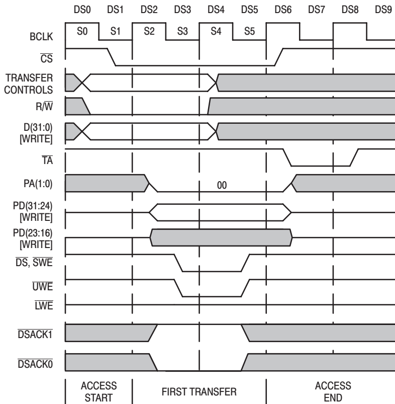
Figure 34. 8-Bit '040 WRITE to 8-Bit Peripheral Example (PA1,PA0=00)
