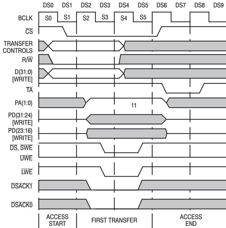
Figure 56. 8-Bit '040 WRITE to 32-Bit Peripheral Example (PA1,PA0=11)
