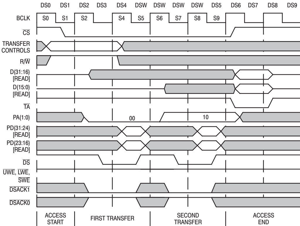
Figure 15. 32-Bit '040 READ From 16-Bit Peripheral Example
