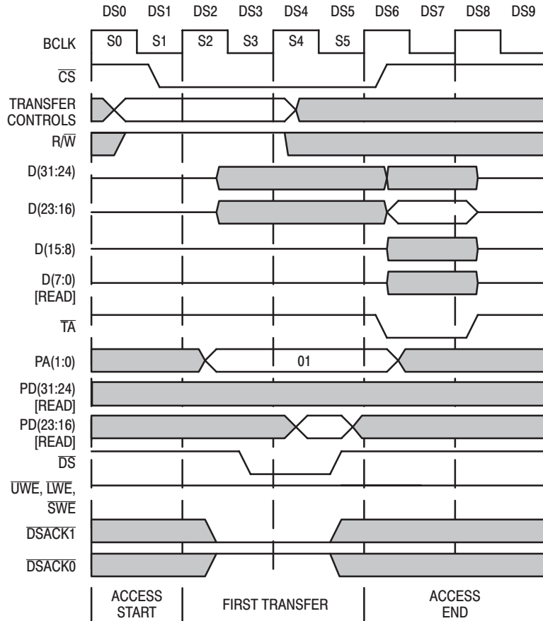
Figure 43. 8-Bit '040 READ From 16-Bit Peripheral Example (PA1,PA0=01)
