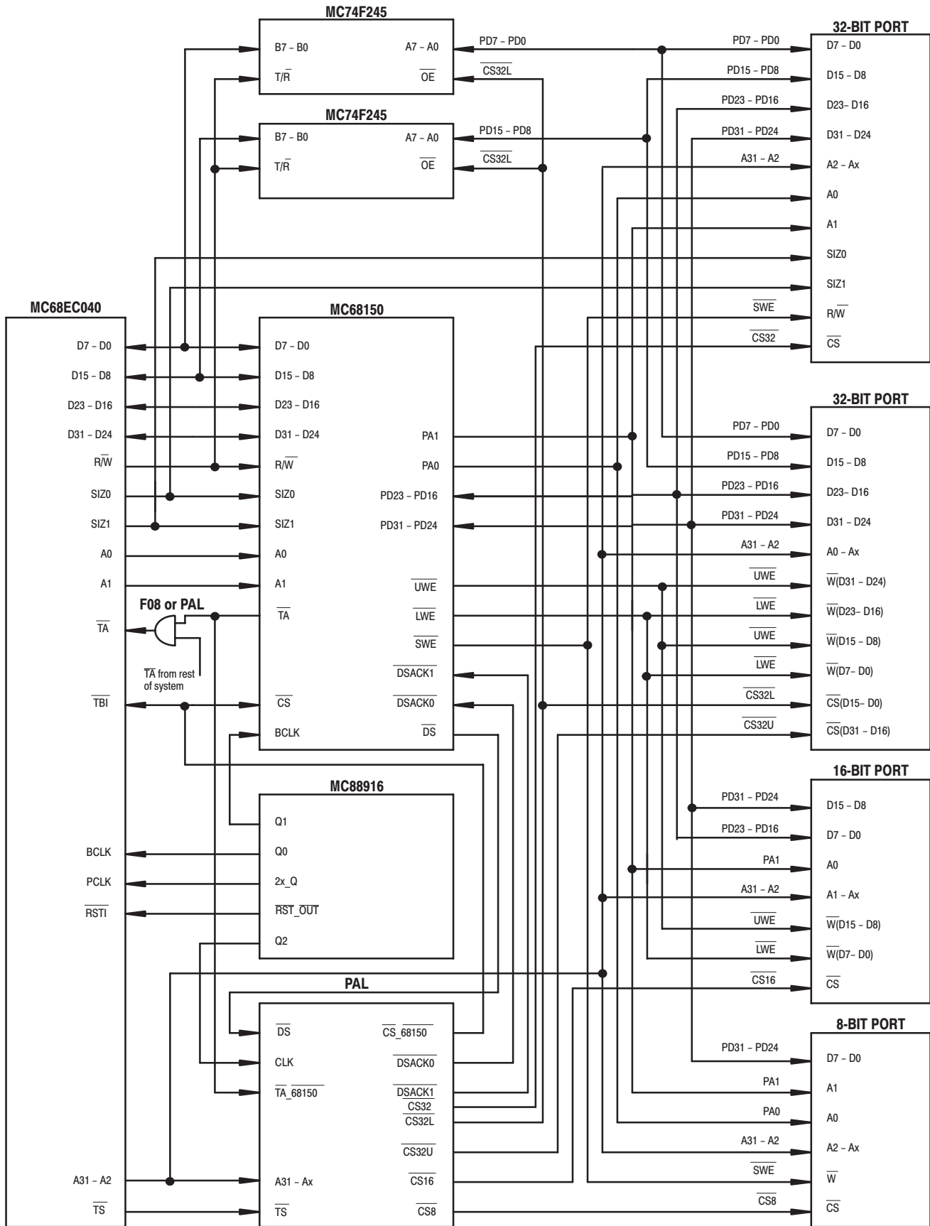
Figure 2. MC68150 Typical System Configuration
