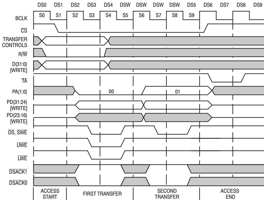
Figure 22. 16-Bit '040 WRITE to 8-Bit Peripheral Example (PA1=0)
