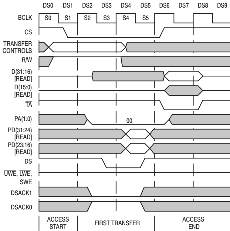
Figure 25. 16 Bit '040 READ From 16-Bit Peripheral Example (PA1=0)
