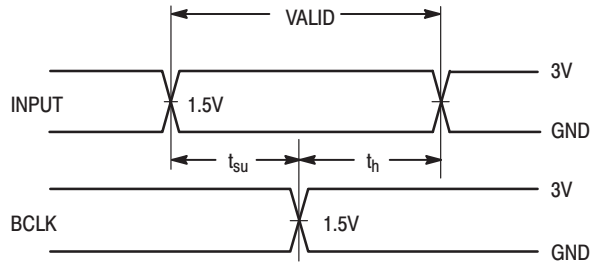
Figure 11. Setup/Hold Times
