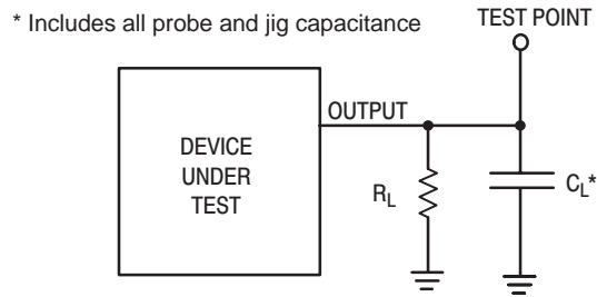
Figure 12. Test Circuit
