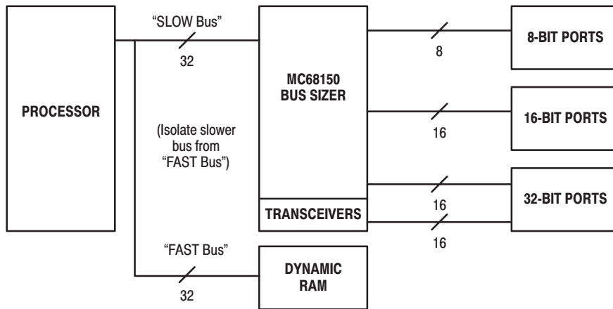
Figure 3. "FAST Bus" "SLOW Bus" Application
