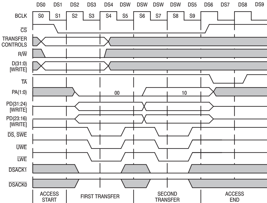
Figure 16. 32-Bit '040 WRITE to 16-Bit Peripheral Example
