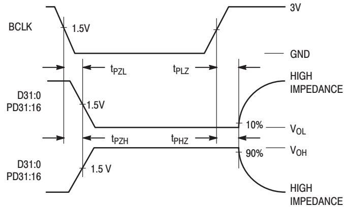
Figure 10. Enable/Disable Times
