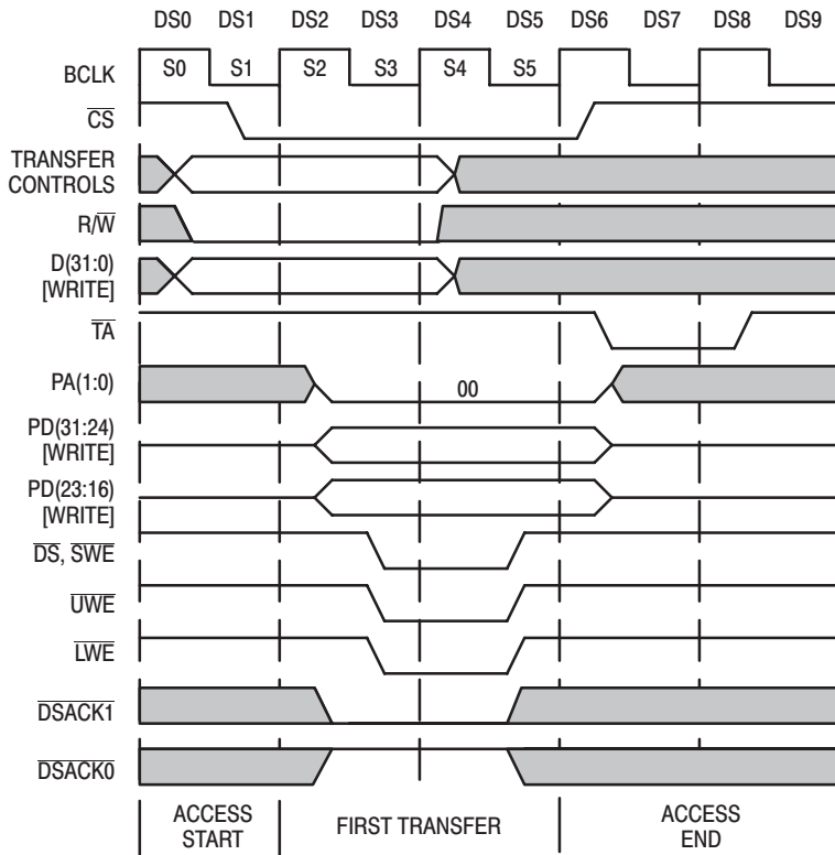
Figure 26. 16-Bit '040 WRITE to 16-Bit Peripheral Example (PA1=0)
