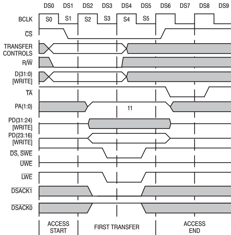
Figure 48. 8-Bit '040 WRITE to 16-Bit Peripheral Example (PA1,PA0=11)
