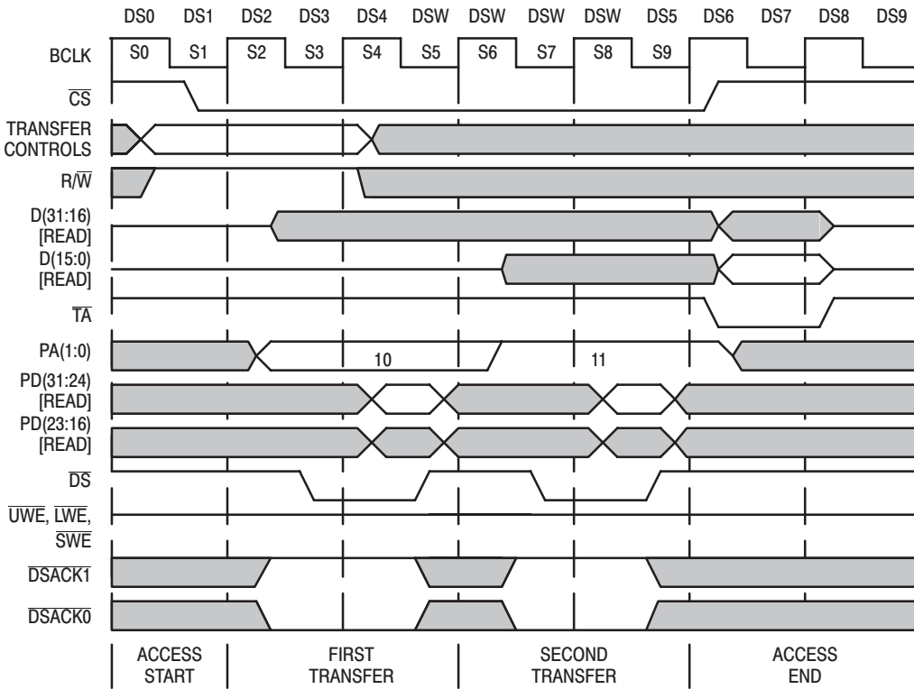
Figure 23. 16-Bit '040 READ From 8-Bit Peripheral Example (PA1=1)
