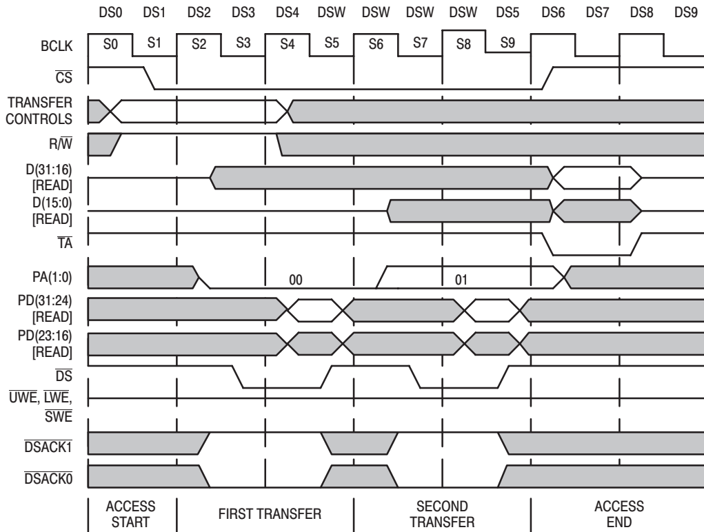
Figure 21. 16-Bit '040 READ From 8-Bit Peripheral Example (PA1=0)
