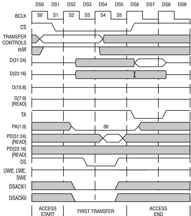
Figure 49. 8-Bit '040 READ From 32-Bit Peripheral Example (PA1,PA0=00)
