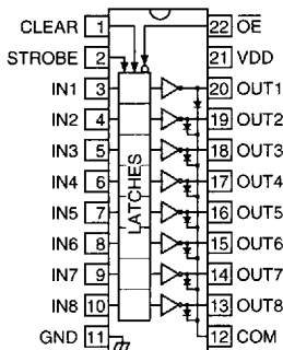
MIC5801BN, AJ
