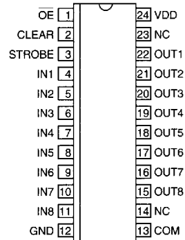
MIC5801BWM
