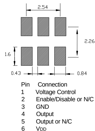
Recommended Pad Layout
