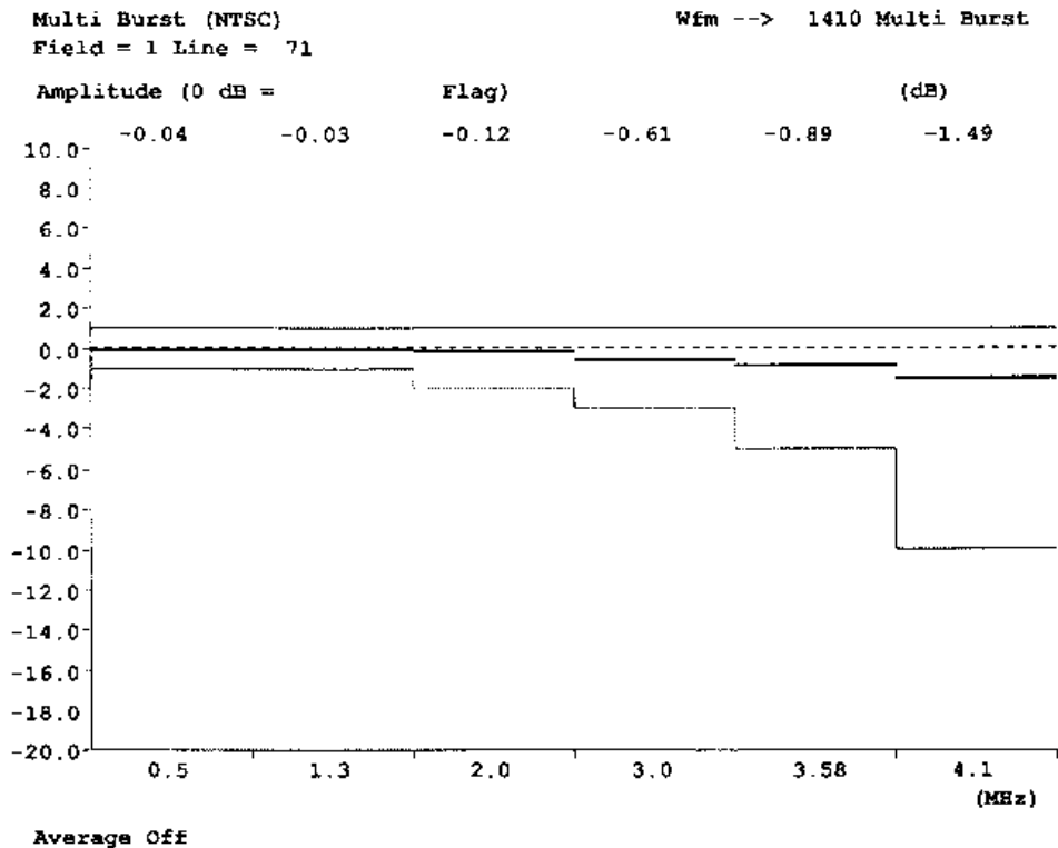
FIGURE 24. MULTIBURST VM700 FREQUENCY ROLL-OFF TEST
