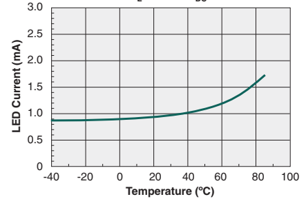
Typical I_F for Switch Dropout vs. Temperature ( I_L=100\text{mA}_{\text{DC}} )
