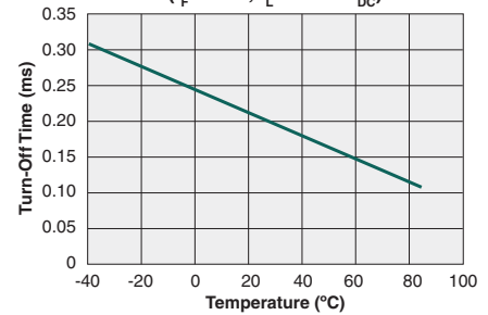
Typical Turn-Off Time vs. Temperature ( I_F=5\text{mA} , I_L=100\text{mA}_{\text{DC}} )
