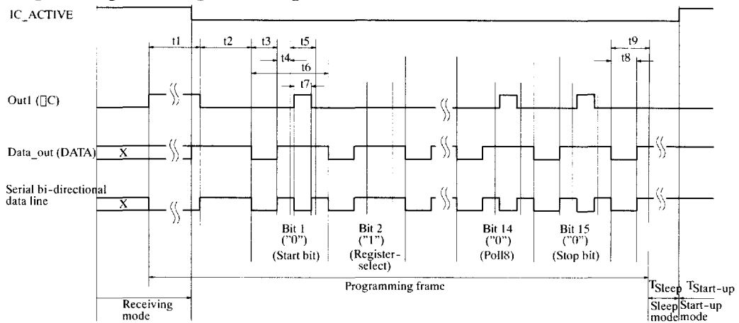
Figure 31. Timing of the register programming
