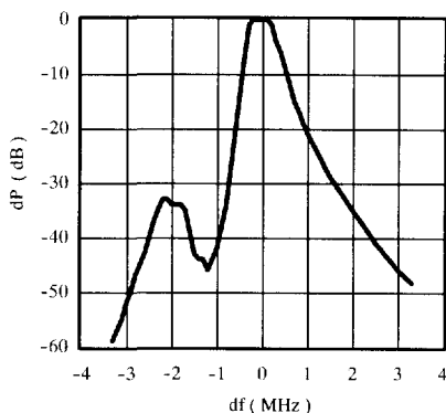
Figure 6. Narrow band receiving frequency response
