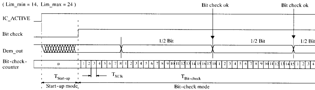
Figure 11. Timing diagram during bit check
