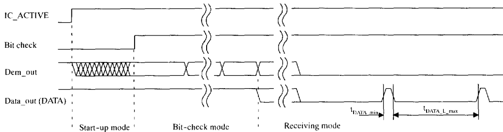
Figure 15. Debouncing of the demodulator output
