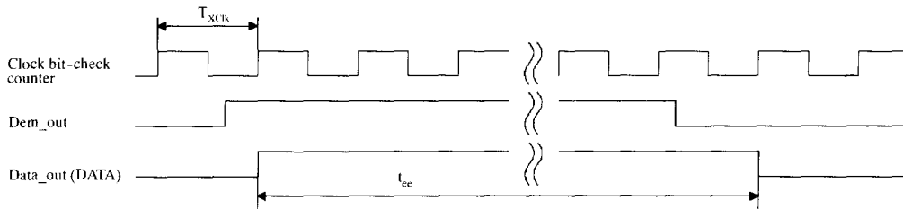
Figure 14. Synchronization of the demodulator output
