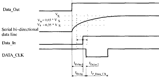
Figure 24. Timing characteristic of the data clock (rising edge on Pin DATA)
