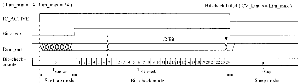
Figure 13. Timing diagram for failed bit check (condition: CV\_Lim \geq Lim\_max )
