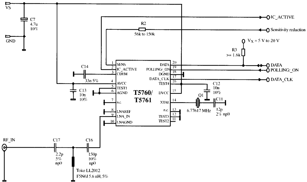
Figure 33. Application circuit: f_{RF} = 868.3 MHz without SAW filter
