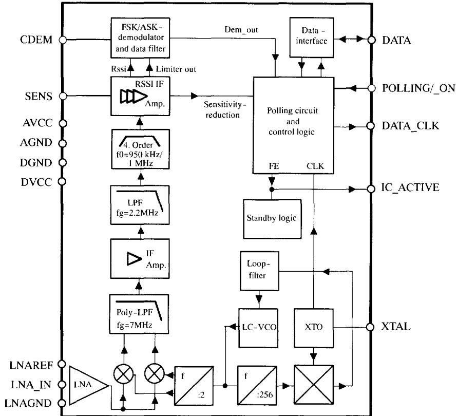
Figure 3. Block diagram
