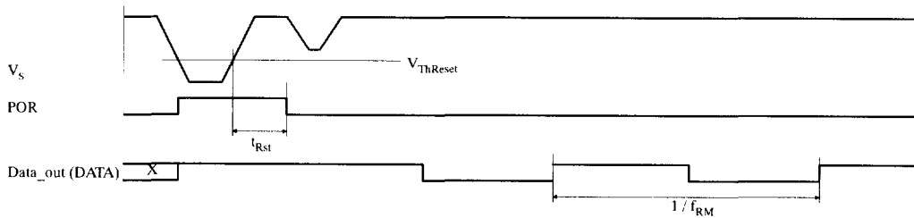
Figure 30. Generation of the power-on reset
