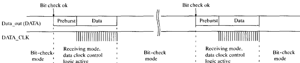
Figure 27. Automatic noise suppression
