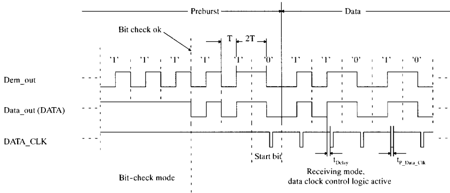
Figure 20. Timing diagram of the data clock
