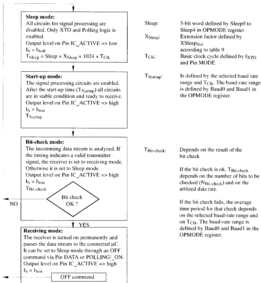
Figure 8. Polling mode flow chart
