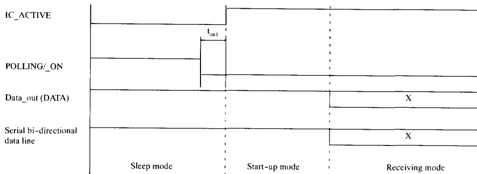
Figure 19. Activating the receiving mode via Pin POLLING/_ON
