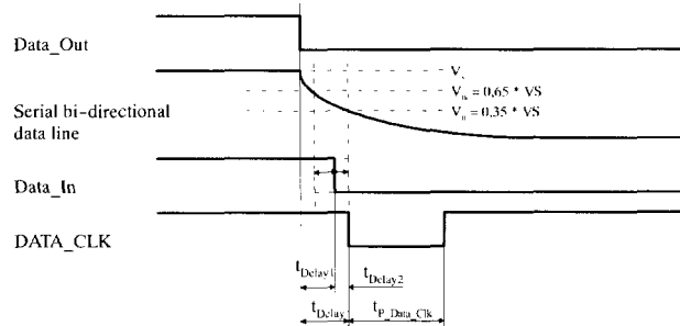
Figure 25. Timing characteristic of the data clock (falling edge of the Pin DATA)
