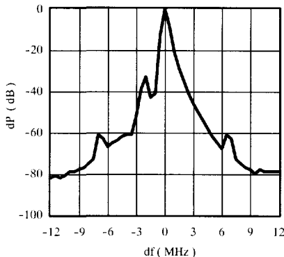
Figure 7. Wide band receiving frequency response
