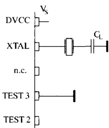
Figure 4. XTO peripherals
