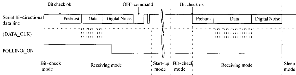
Figure 29. Controlled noise suppression
