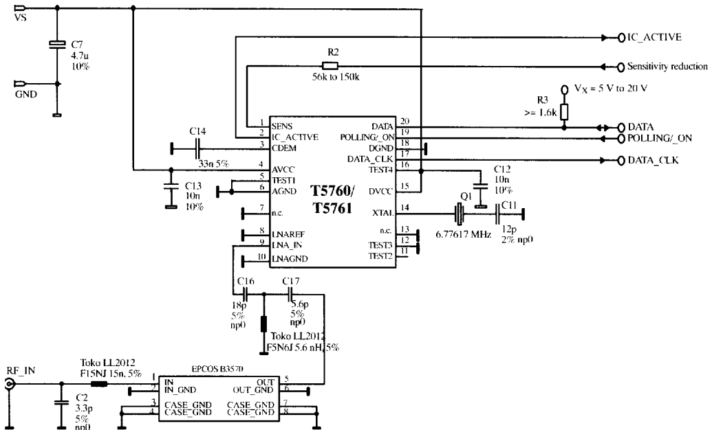
Figure 34. Application circuit: f_{RF} = 868.3 MHz with SAW filter
