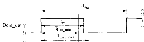
Figure 10. Valid time window for bit check
