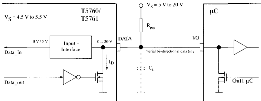
Figure 32. Data interface
