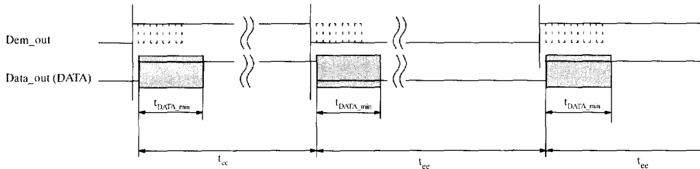
Figure 14. Synchronization of the demodulator output
