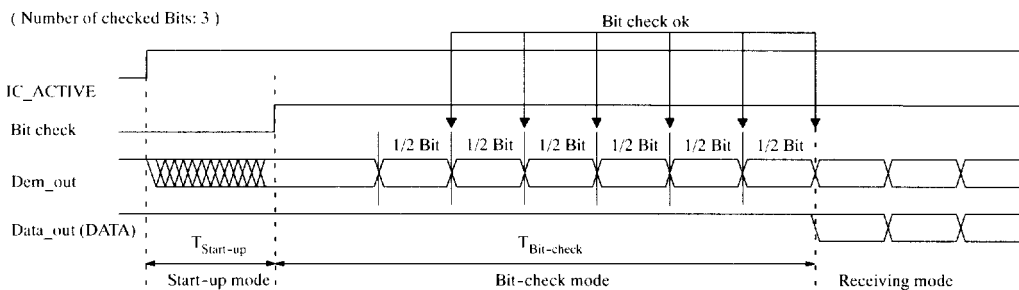
Figure 9. Timing diagram for complete successful bit check
