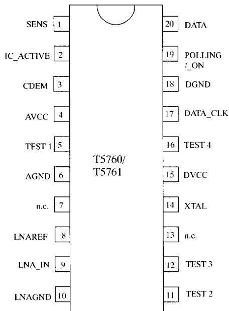
Figure 2. Pinning SO20
