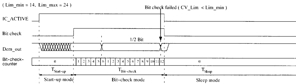
Figure 12. Timing diagram for failed bit check (condition: CV\_Lim < Lim\_min )
