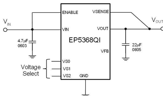
Figure 2. Typical Application Schematic
