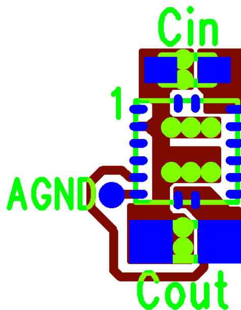
Figure 8. Top PCB Layer Critical Components and Copper for Minimum Footprint
