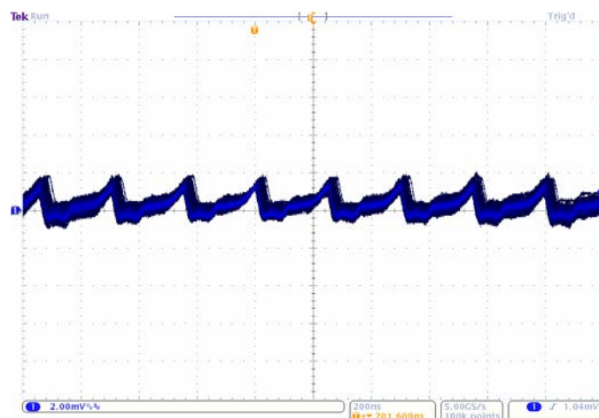
Voltage Ripple, V_{IN} = 3.3V , V_{OUT} = 1.8V , Load = 600mA C_{OUT} = 2 \times 10\mu F , 0805, 2.0mV/Div.
