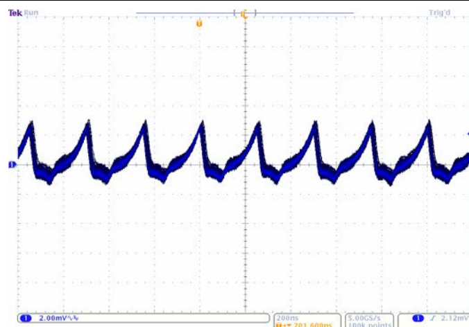
Voltage Ripple, V_{IN} = 3.3V , V_{OUT} = 1.8V , Load = 600mA C_{OUT} = 1 \times 22\mu F , 0805, 2.0mV/Div.
