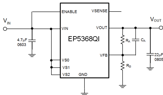
Figure 7. Applications Circuit for Operation at 700mA
