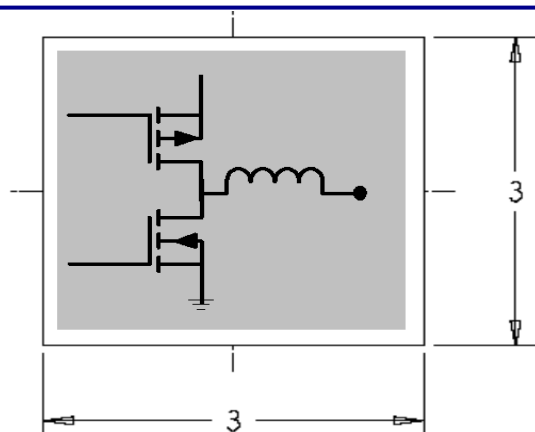
Figure 1. Features Integrated Inductor Technology
