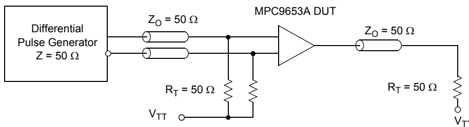
Figure 9. PCLK MPC9653A AC test reference
