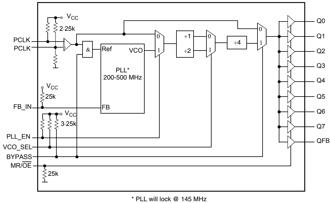
Figure 1. MPC9653A Logic Diagram
