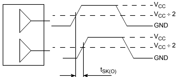
Figure 10. Output-to-output Skew t_{SK(O)}
