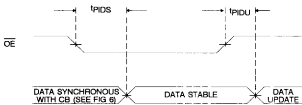
FIGURE 7 Inhibiting Output Data Update
