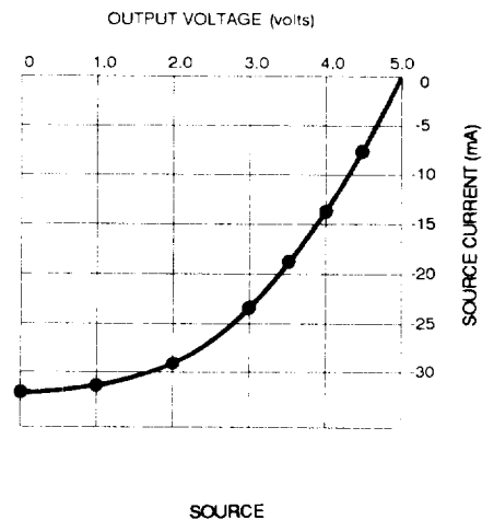
FIGURE 11 Output Drive Current (Typical @ V_L = 5\text{ V-dc} , T_a = 25^\circ\text{C} )
