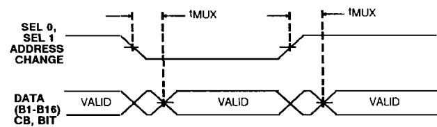
FIGURE 10 Output Select Time
