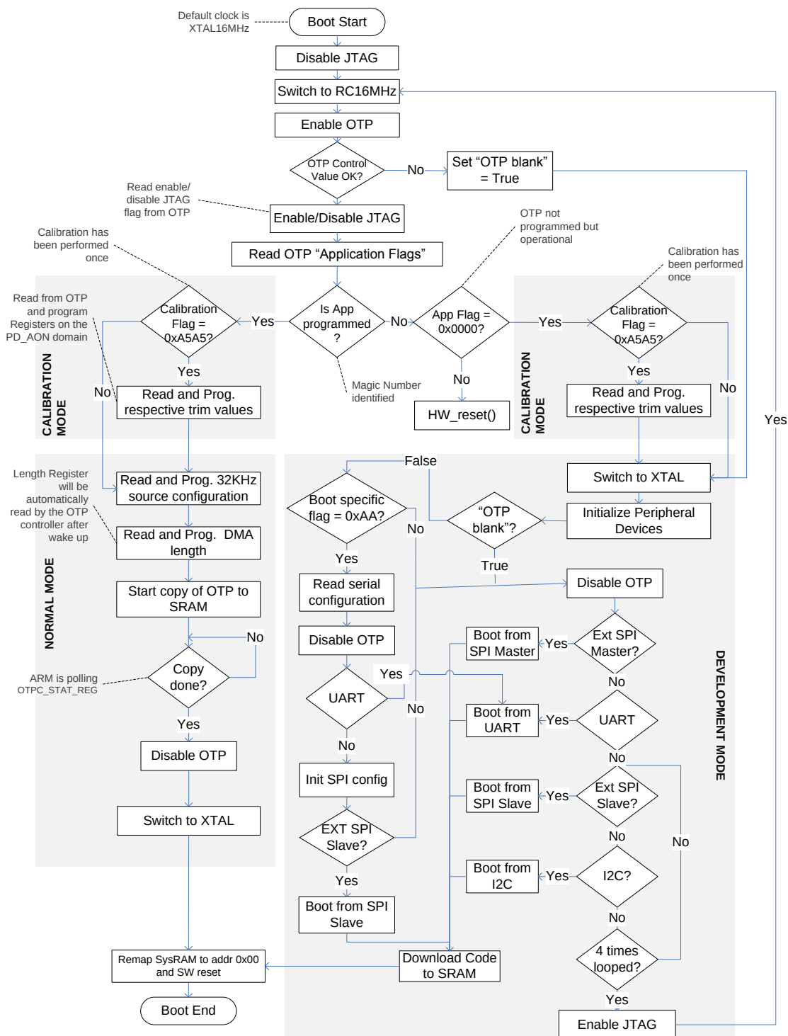
Figure 9: BootROM Sequence
