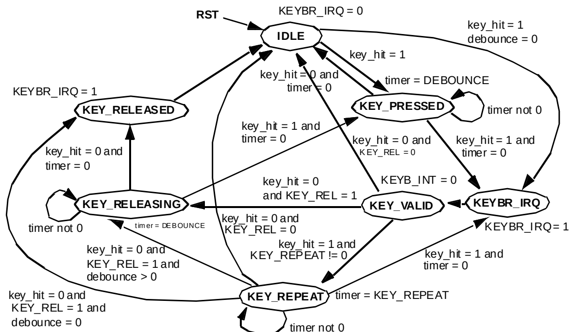
Figure 59: Keyboard Scanner State Machine
