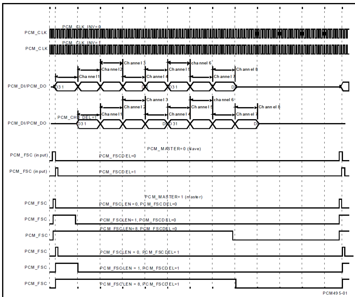
Figure 65: PCM Interface Formats
