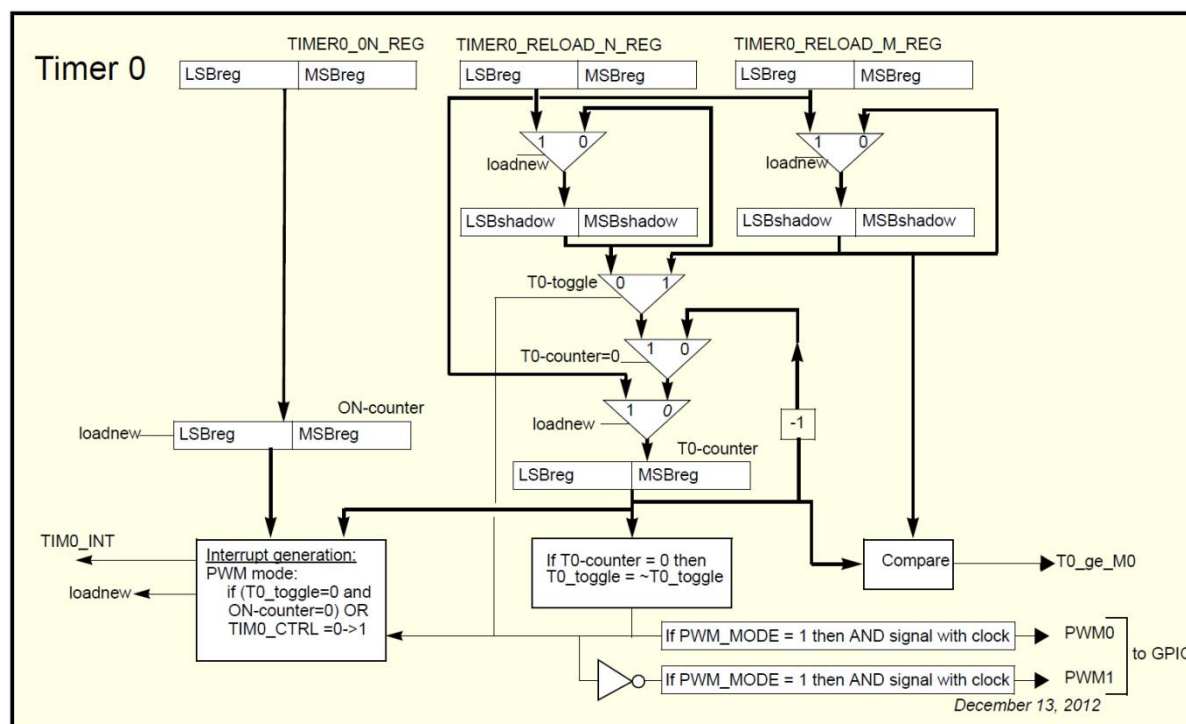
Figure 53: Timer 0 Block Diagram
